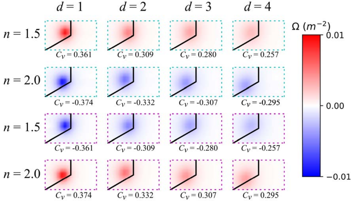
FIG. 4. The Berry curvature distributions around K_6 point. Berry curvature distributions for the second band (upper two rows enclosed by the cyan dotted boxes) and for the third band (lower two rows enclosed by the magenta dotted boxes) are shown with different parameters. The color represents the amplitude of the Berry curvature (see the colormap), and the black lines are the boundaries of the Brillouin zone. Given that the side length of the first Brillouin zone is S_{BZ} , the width of the area is \frac{1}{2}S_{BZ} , and the height of the area is \frac{1}{2}S_{BZ} .
