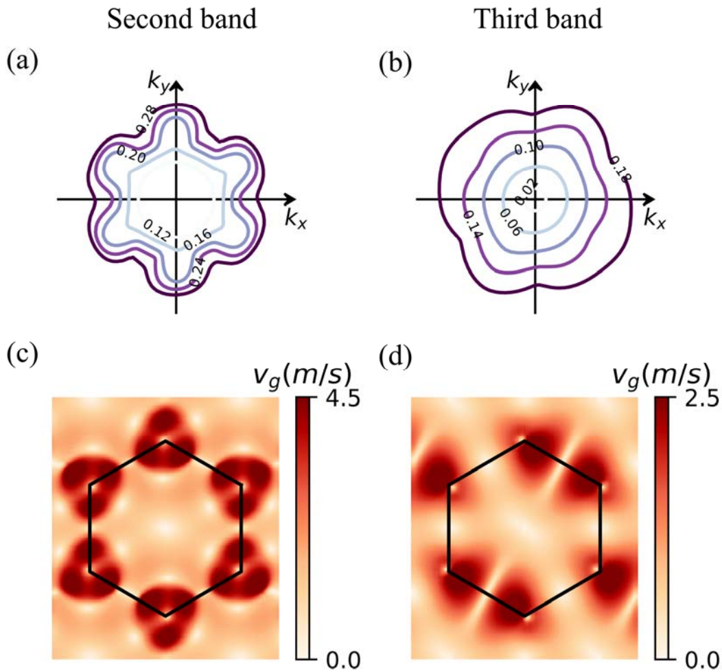
FIG. 3. (a) The slowness curves of the second band. From the small wave vectors to large wave vectors, the slowness rises from 0.12 to 0.28. (b) The slowness curves of the third band. From the
