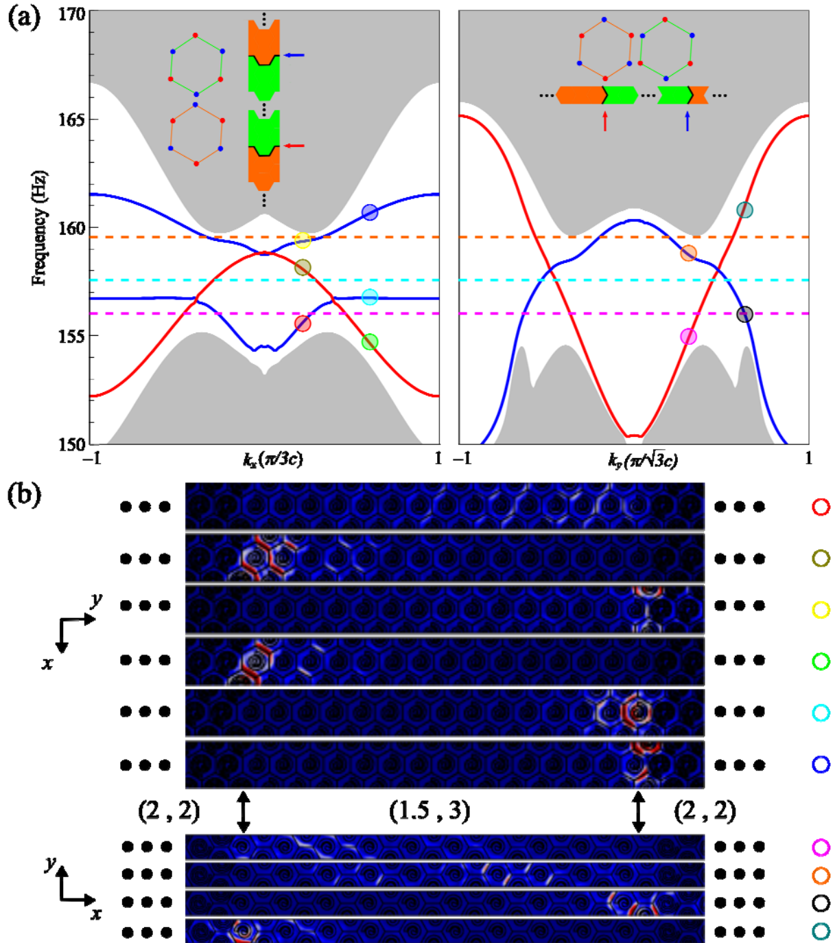
FIG. 6. (a) The projected band structures along the \mathbf{k}_x (left panel) and \mathbf{k}_y (right panel) directions. Several markers with different colors are shown in the topological band. For the projected band structure along the \mathbf{k}_x direction, markers are placed on each topological band at k_x = 0.26 and k_x = 0.6 . For the projected band structure along the \mathbf{k}_y direction, markers are placed on each topological band at k_y = 0.3 and k_y = 0.6 . The schematics of supercell setup are displayed as the
