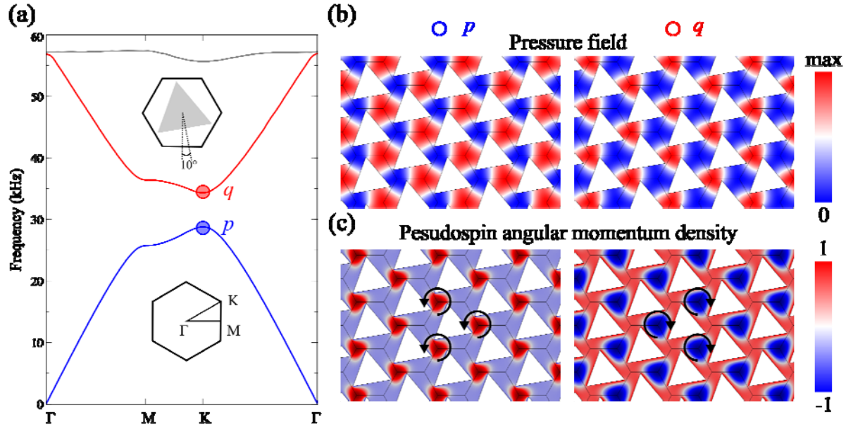
FIG. 8. (a) The band structure along \Gamma -M-K- \Gamma of the acoustic valley metamaterial for comparison. The blue, red and gray curves represent the first, second and third bands, respectively. (b) The amplitude distributions of pressure fields of the p and q states. (c) The normalized pseudospin angular momentum density of the p and q states.
