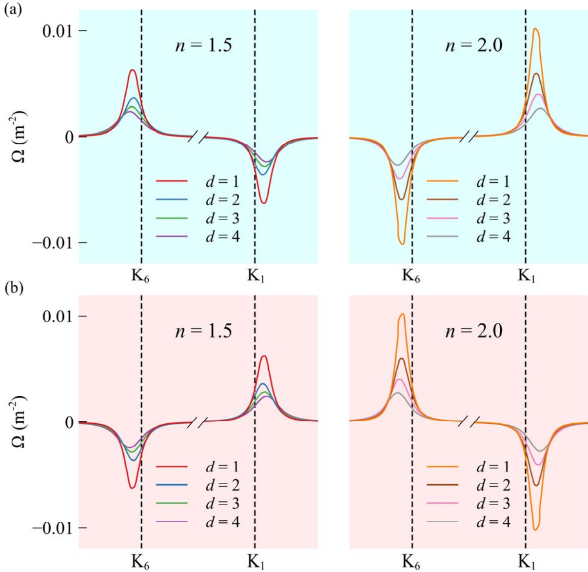
FIG. 5. (a) The Berry curvature of the second band along K_6 K_1 line as a function of the thickness of the Archimedean spiral, d = 1, 2, 3 and 4 [mm], when the number of turns of the spiral n = 1.5 and 2 . (b) The same for the third band. Note that there is a broken x axis in each figure to emphasize the change of the Berry curvature in the K points.
