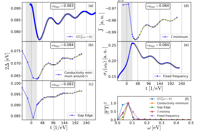
FIG. 4. (Color online) The Higgs oscillation. The figure shows the dynamics of the superconducting order parameter in a pump induced non-equilibrium state (for A_{\max} = 0.2 [1/a 0 ]). Panel (a) shows the order parameter as a function of average time calculated using anomalous self-energy. Panels (b) and (c) display the estimated order parameter using the location of the minimum of the real part of optical conductivity around the phonon frequency (shown in the blue shaded region II in figure 3) and the gap edge location (the red shaded region I in figure 3), respectively. Panel (d) and (e) show the probe current minimum and \sigma_1(\omega = 0.09) as a function of time, respectively. All the five quantities shown in panels exhibit oscillations in time with approximately same frequency ( \omega_{\text{Higgs}} \approx 2\Delta(t) ), which is calculated by fitting the data to an oscillatory decaying function. The Fourier transform of the data also shows a peak at the same frequency (panel (f)).
