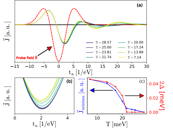
FIG. 2. (Color online) Probe current in equilibrium state. Panel (a) shows the probe current as a function of time at different temperatures in equilibrium. The temperature-range spans the superconducting phase transition. Panel (b) displays the zoomed region around the global minimum of the probe current. Panel (c) shows the correlation between the probe-current minimum and the superconducting order parameter calculated using \Sigma_R^F(\omega = 0) .
