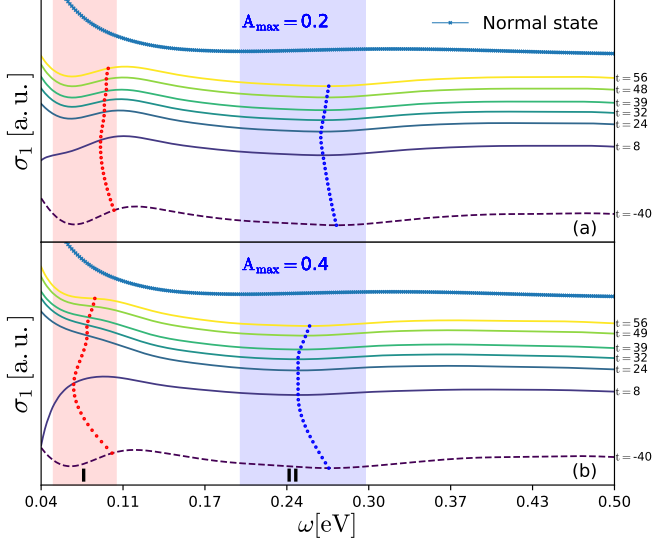
FIG. 3. (Color online) Conductivity of the system in a pump driven non-equilibrium state. Panel (a) and (b) show the real part of optical conductivity as a function of frequency at different delay times for pump fluence A_{\max} = 0.2 [1/a 0 ] and 0.4 [1/a 0 ]. Each curve is shifted by an offset (scaled as the delay time) along Y-axis to show the changes in the transient conductivity. The top dashed line in each panel shows the conductivity of normal state in equilibrium. Conductivity of the superconducting state is shown by t = -40 [1/eV] in equilibrium. The blue shaded region II shows the vicinity where the location of the \sigma_1 minimum resides near the phonon frequency \Omega . The minima are shown by the dotted curve connecting different delay-time curves. The red shaded region I shows the region where the gap edge is located and marked by the dotted line connecting different delay-time curves.
