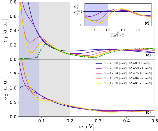
FIG. 1. (Color online) The conductivity of the Holstein model in equilibrium. Panels (a), (b) show the real and the imaginary part of optical conductivity at different temperatures, respectively. The temperature-range spans the superconducting phase transition. The dark shaded region shows the maximum superconducting optical gap near zero temperature 2\Delta(T \approx 0) . The light shaded region shows the phonon window ( 0 < \omega < \Omega = 0.2 eV). Panel (c) displays the ratio of real parts of conductivity in the superconducting state to normal state at T = 25 meV. The dashed line in panel (a) shows \sigma_1 calculated using bare-bubble susceptibility at T = 12.2 [meV].
