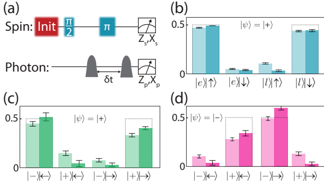
FIG. 8. (a) Experimental sequence for generating and verifying spin-photon entanglement. A time-bin encoded qubit is reflected by the cavity, and both the SiV and the photonic qubits are measured in the Z and X bases. (b) Spin-photon correlations measured in the Z-Z basis. Light (dark) bars are before (after) correcting for known readout error associated with single-shot readout of the SiV. (c) Spin-photon correlations measured in the X-X basis. Bell-state preparation fidelity of F \geq 0.89(3) and a concurrence \mathcal{C} \geq 0.72(7) . (d) Preparation of second spin-photon Bell state. Changing the phase of the incoming photonic qubit prepares a Bell-state with inverted statistics in the X basis.
