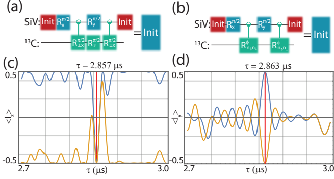
FIG. 13. (a) Original initialization sequence from [65], note \mathcal{R}_{z,C}^{\pi/2} rotation. (b) Simplified initialization sequence used in this work. (c) Simulated performance of the initialization gate from (b) using 8 \pi -pulses per each nuclear gate, the initial state is |\uparrow\uparrow\rangle (blue) and |\uparrow\downarrow\rangle (orange). The resonances are narrow compared to (d) due to applying effectively twice more \pi -pulses (d) Simulated performance of \mathcal{R}_{\pm x, \text{SiV-C}}^{\pi/2} gate for 8 \pi -pulses for SiV- ^{13}\text{C} register initialized in |\uparrow\uparrow\rangle (blue) and |\uparrow\downarrow\rangle (orange)
