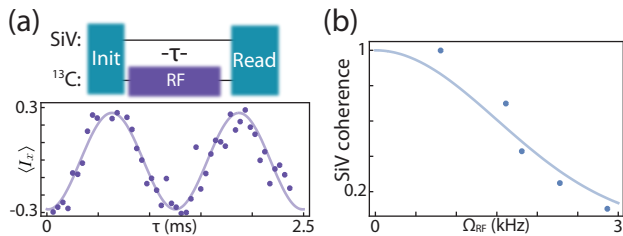
FIG. 10. (a) RF Rabi oscillations. Applying an RF tone directly drives nuclear rotations of a coupled ^{13}\text{C} . (b) SiV coherence in the presence of an RF drive. As the strength of the RF drive is increased, local heating from the CPW reduces the SiV T_2 .
