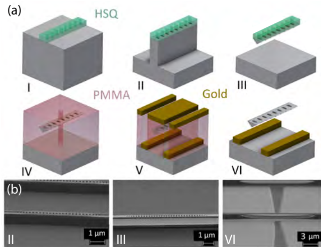
FIG. 2. (a) Schematic of the nanofabrication process used to produce devices. I: HSQ mask with a 10 nm titanium adhesion layer is patterned using EBL. II: Pattern is transferred onto diamond using top down \text{O}_2 RIE. III: Angled IBE is used to separate structures from substrate. IV: Devices are covered in PMMA and implantation apertures are formed using EBL. Device are then cleaned, implanted, and annealed. V: PMMA is used in a liftoff procedure to pattern gold microwave striplines. VI: Final devices are cleaned and prepared for experiment. (b) Scanning electron micrographs corresponding to steps II, III, and VI in the fabrication procedure.
