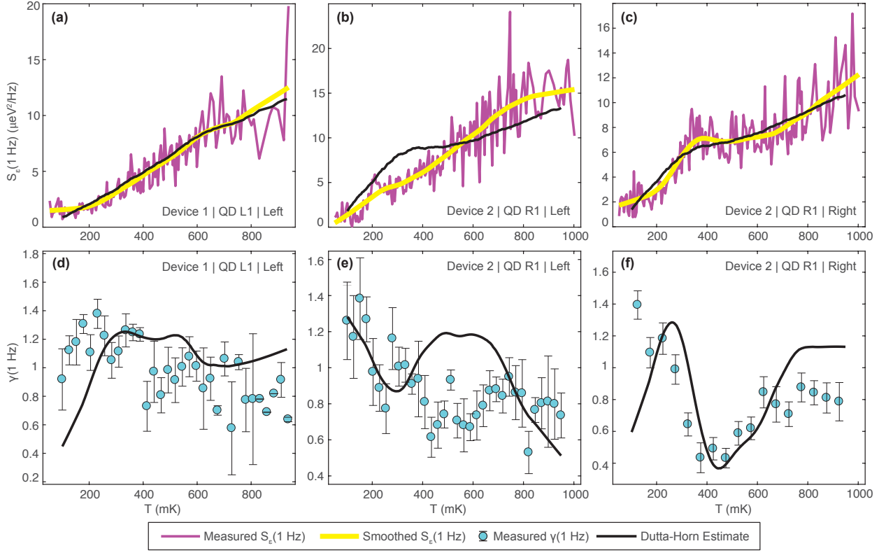
Fig. 4 Measured temperature dependence of the noise magnitude and exponent. a S_\epsilon(1 \text{ Hz}) versus temperature on the left side of a transport peak for quantum dot L1 on device 1. b S_\epsilon(1 \text{ Hz}) versus temperature on the left side of a transport peak for dot R1 on device 2. c S_\epsilon(1 \text{ Hz}) versus temperature on the right side of the transport peak for dot R1 on device 2. d Averaged measurements of \gamma(1 \text{ Hz}) versus temperature on the left side of the transport peak for dot L1 on device 1. e Averaged measurements of \gamma(1 \text{ Hz}) versus temperature on the left side of the transport peak for dot R1 on device 2. f Averaged measurements of \gamma(1 \text{ Hz}) versus temperature on the right side of the transport peak for dot R1 on device 2. The smooth yellow lines are generated by taking a moving average of the data. The black lines in a , b , and c are the estimates for S_\epsilon(1 \text{ Hz}, T) using Equation 6 of the Dutta-Horn model and the data in d , e , and f , respectively. Error bars in d , e , and f represent the standard error associated with averaging the data over temperature ranges of 25 mK. The solid lines in d , e , and f are estimates for \gamma(1 \text{ Hz}, T) using Equation 6 of the Dutta-Horn model and the smoothed yellow lines in a , b , and c , respectively.
