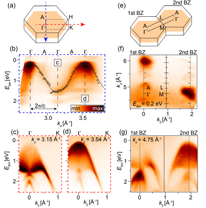
FIG. 3. (color online) ARPES measurements of the k_z -dispersion of GaSe. (a) Sketch of bulk BZ highlighting the \Gamma - A - H - K plane. (b) Dispersion along the \Gamma - A direction, as marked by the blue dashed line in (a). Fits of the position of the VBM intensity are shown via open circles. The solid curve following the fitted dispersion is a guide for the eye. The BZ size of 2\pi/c in the z -direction is marked by a double-headed arrow and two vertical dashed lines. (c)-(d) Dispersion extracted at the given k_z values, corresponding to the \Gamma - K direction (red dashed line). (e) Sketch of 1st and 2nd BZs with an outline of the \Gamma - A - L - M plane. (f) Constant energy contour of the plane sketched in (e) extracted at a binding energy of 0.2 eV with high symmetry points annotated by tick marks. (g) Dispersion along the \Gamma - M - \Gamma direction obtained at a k_z value of 4.75 \text{ \AA}^{-1} .
