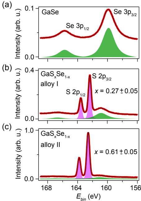
FIG. 5. (color online) Composition of \text{GaS}_x\text{Se}_{1-x} alloys from core level data. (a)-(c) Core level measurements (red thick curves) in the Se 3p and S 2p binding energy region for (a) GaSe and (b)-(c) \text{GaS}_x\text{Se}_{1-x} alloys. Fit results (black curves) to Doniach-Sunjić line shapes (filled peaks) are provided in each panel. The composition x of the alloys determined via the fitted peak components is stated in (b)-(c). Note the intensity scale varies between the panels.
