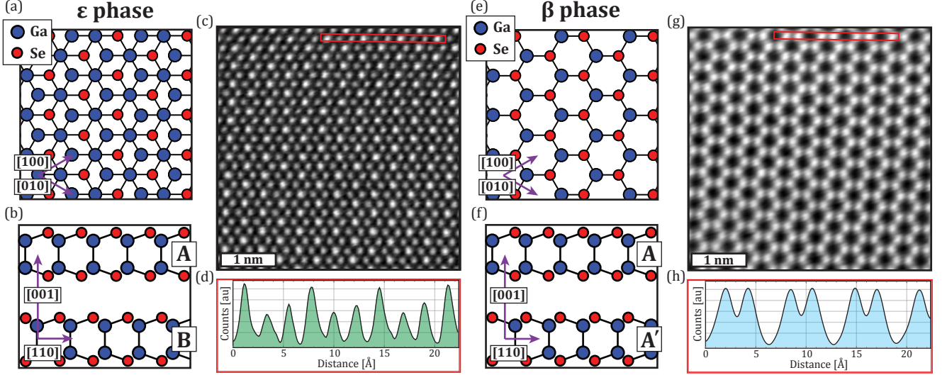
FIG. 1. (color online) Real space structure and HRSTEM images of the two most common \text{GaS}_x\text{Se}_{1-x} polytypes. Panels (a) and (b) show the crystal structure of the \epsilon phase in the planes defined by the axes in the labels. The corresponding HRSTEM image in (c) shows a trigonal lattice, resulting from the projection of Bernal (AB) stacked honeycomb layers. The intensity cut in (d) was obtained from the red rectangle in (c) and shows bright atomic columns with approximately twice the intensity of dim atomic columns. Analogous images in (e)-(f) show the geometry of the \beta phase. The HRSTEM image in (g) shows a honeycomb mesh, with no intensity in the interstitial columns between hexagonal cells.
