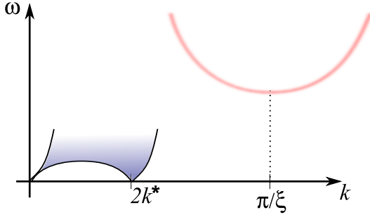
FIG. 3. (color on-line) The spin response of the KL close to the special commensurate fillings. The main response is at frequencies higher than the spin gap and coming from the vicinity of the commensurate wave vector (e.g., \pi/\xi for half filling). The spin response of TLL is shifted to the region of wave vectors between 0 and 2k_F^*
