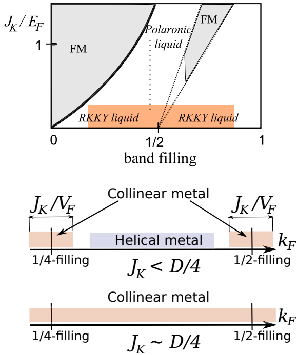
FIG. 1. (color on-line) The upper panel: a cartoon illustrating the weak and the moderate coupling regimes of the phase diagram obtained numerically for 1D KL in Ref. 19 . The two shaded regions are ferromagnetic phases. The region called “Polaronic Liquid” corresponds to the large Fermi surface whose volume incorporates both conduction and localized electrons. The Kondo effect is suppressed in all regions. The orange box marks the range of parameters considered in the present paper. The central and the lower panels: phase diagrams of 1D KL obtained for small J_K/E_F , see explanations in Sect. V
