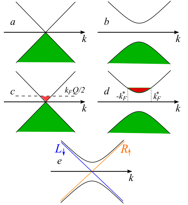
FIG. 2. (color on-line) Panels (a) and (b): the ground state of fermions \tilde{R}, \tilde{L} with zero chemical potential (green region) before and after opening the gap at the level of \mu . Panels (c) and (d): the ground state of the fermions for the case of a finite positive chemical potential. The red regions mark the states between the gap and the chemical potential which can form Tomonaga-Luttinger liquid. Panel (e) exemplifies a co-existence of the gapped (black lines) and the gapless (orange and blue lines) helical fermions.
