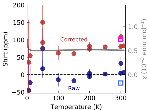
Figure 8. Comparison of the raw and (demagnetization) corrected shift of the ^8\text{Li} NMR in the \text{LaNiO}_3 crystal. The raw shift is obtained by using Eq. (2), while the corrected shift is obtained by applying the demagnetization correction in Eq. (C1). The results at 300 K for the film are shown as open squares. Overlaid on the corrected shifts is the molar susceptibility of the crystal, 15 right scale.
