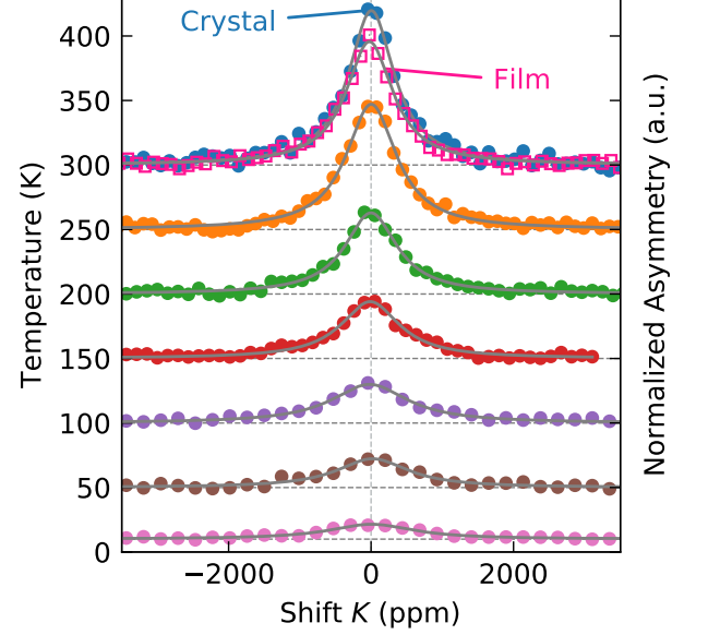
Figure 3. Temperature dependence of the ^8\text{Li} resonance in the \text{LaNiO}_3 crystal at 6.55 T. At low temperature, the resonance is broadest and weakest, with the amplitude growing monotonically and the width narrowing by a factor of \sim 2 as the temperature is raised. A small, nearly temperature independent positive shift relative to \text{MgO} is evident. The spectra are normalized by the off-resonance baseline asymmetry and offset to clearly display the temperature dependence. The ^8\text{Li} resonance in the LNO film at 300 K is also shown (open squares); it is remarkably similar to the crystal both in shift K and width.
