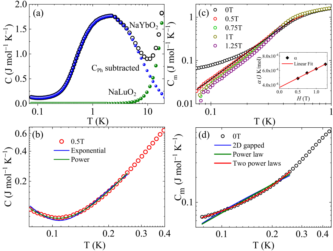
FIG. 3. (a) Specific heat data for NaYbO 2 and the non-magnetic reference NaLuO 2 . It shows that the lattice contribution below 2 K is negligible. (b) Example for the fit of the raw specific-heat data in order to determine the nuclear contribution C_{nucl} . (c) The magnetic contribution C_m = C - C_{nucl} of the specific heat of NaYbO 2 in a double-logarithmic plot in low magnetic fields after subtracting the nuclear contribution. The black line is a guide to the eye and shows that C_m follows a power law only if a magnetic field is applied. The zero-field data clearly deviate from that behavior. The inset shows the field dependence of parameter \alpha and its extrapolation to zero field. (d) Zero-field magnetic specific heat of NaYbO 2 with fits using different functions.
