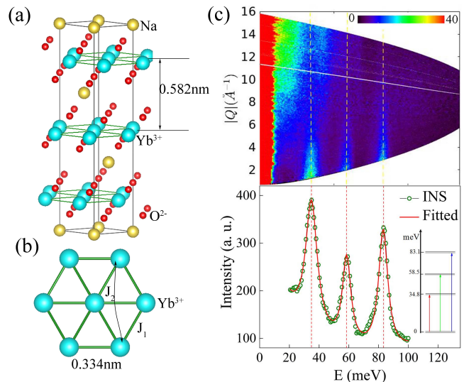
FIG. 1. (a) Stacking of the \text{Yb}^{3+} triangular-layers along the c -axis. (b) Triangular layer formed by \text{Yb}^{3+} cations. (c) Inelastic neutron scattering spectra S(Q, \hbar\omega) at 5 K with E_i=150 \text{ meV} . Energy dependence of the INS intensity at 5 K integrated in Q over the range 3.9\text{-}4.4 \text{ \AA}^{-1} . Inset depicts the CEF transitions from the ground-state Kramers doublet.
