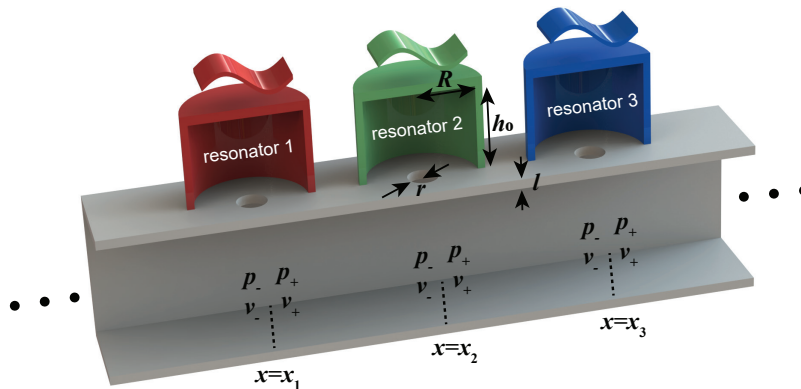
FIG. 1: Schematic representation of a waveguide loaded with arbitrary number of space-time modulated resonators
