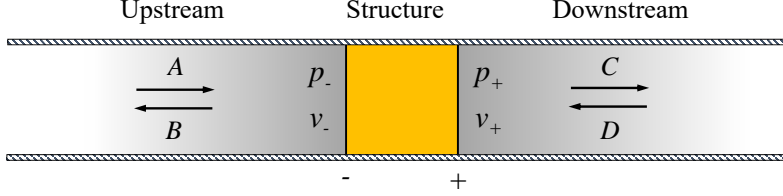
FIG. B1: Schematic of the system for matrix conversion.
