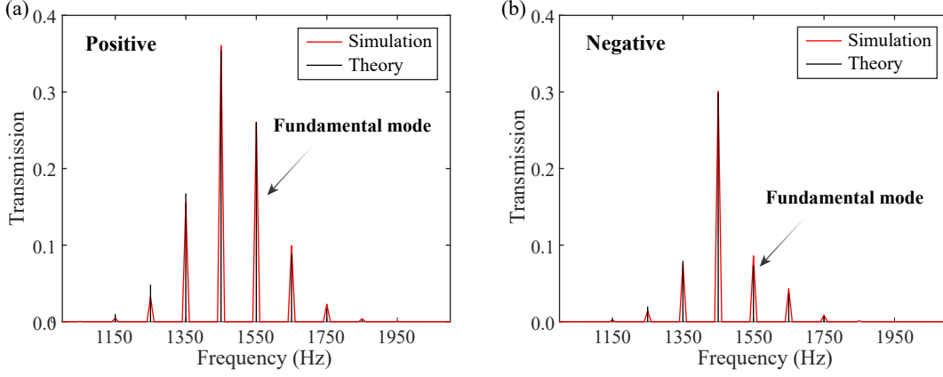
FIG. 3: Comparison of the transmission coefficients for each order between theoretical calculation and FDTD simulation. The amplitudes of all the involved orders agree well. Non-reciprocal sound transport is achieved at the fundamental frequency of 1550 Hz.
