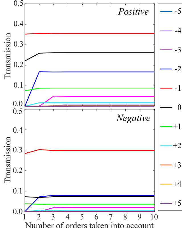
FIG. C1: Transmission coefficients for 0 to \pm 5 order modes as we increase the number of orders taken into account. (a) and (b) showed the scenario when the incident wave is from positive direction and negative direction, respectively. The results remain unaffected after accounting for the \pm 5 order.
