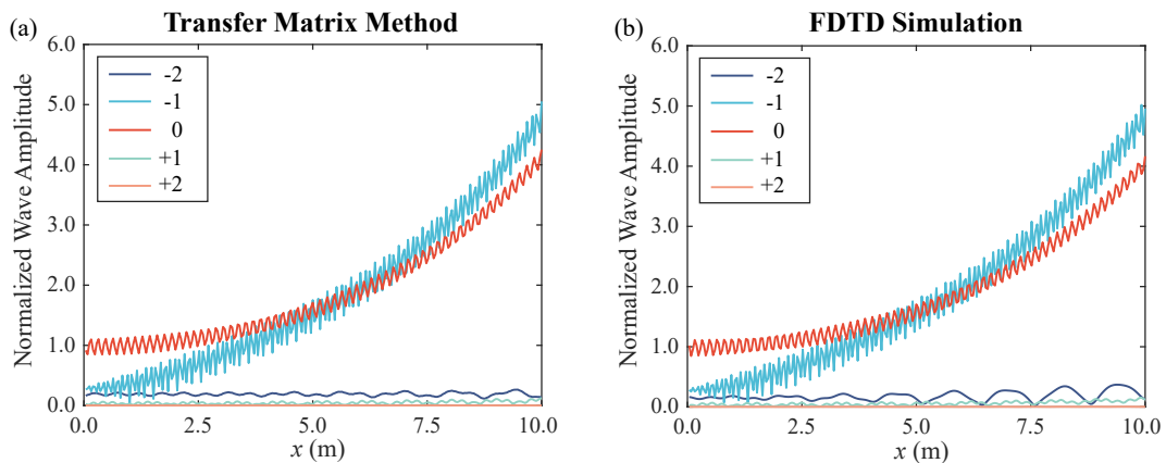
FIG. 5: Comparison between theory and simulation for the case of parametric amplification (non-Hermitian gain media). (a) The wave amplitudes for 0 to \pm 2 nd order waves along the waveguide predicted by the transfer matrix method. The calculation truncated at \pm 10 th order. (b) Amplitudes for 0 to \pm 2 th order waves obtained from simulation.
