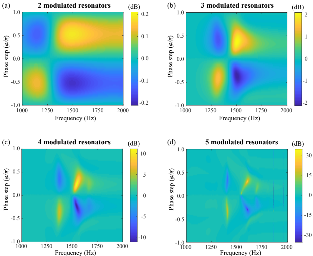
FIG. 2: Transmission ratio for 2, 3, 4 and 5 space-time modulated resonators with the change of input frequency and modulation phase step. With the increased number of resonators, the range of available transmission ratio can be increased.
