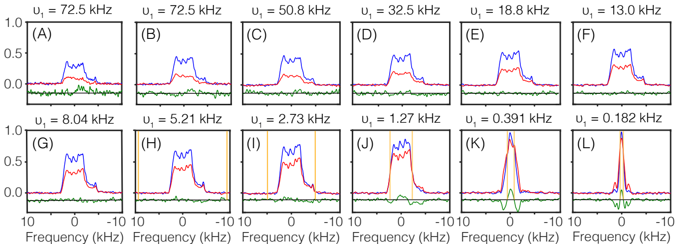
FIG. 2. Comparison of the ^{17}\text{O} MAS NMR spectra of polycrystalline coesite at 9.4 T from the 1 st and 15 th echoes obtained with CPMG using square pulses for different rf field strengths as indicated above each spectrum. Echo 1 is depicted in blue, echo 15 is depicted in red, the residual difference between the two after renormalizing intensities is depicted in green, and the sinc excitation profile FWHM is depicted in orange. For powers above \omega_1/(2\pi) = 5.21 kHz, the excitation profile FWHM is wider than the plot's window. In (A) the \pi/2 and \pi pulse lengths of 1.8 \mu\text{s} and 3.4 \mu\text{s} , respectively, were determined from the first maximum and null of a nutation measurement on the coesite ^{17}\text{O} signal. In (B)-(L) the \pi/2 and \pi pulse lengths were then set to the theoretical values of \pi/(6\omega_1) and \pi/(3\omega_1) , respectively, for the central transition of the I = 5/2 nucleus. All \pi pulses had a spacing of 8 ms. Further experimental details are given in the supplemental material[9].
