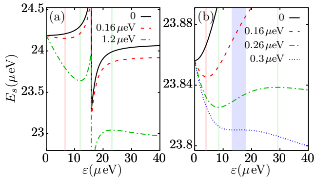
Figure 3. Spin qubit energy splitting E_s as a function of the detuning \varepsilon , for various values of the longitudinal gradient field ( g\mu_B b_z ), as indicated, increasing from top to bottom. The interdot tunnel splitting amounts to (a) 2t_c = 18 \mu\text{eV} and (b) 2t_c = 30 \mu\text{eV} , while the homogeneous field Zeeman energy is E_z = 24 \mu\text{eV} and the transverse inhomogeneous component is g\mu_B b_x = 2 \mu\text{eV} . The thin shaded areas indicate first order sweet spots for the corresponding color line and the wide blue shaded area in (b) indicates the region around the second order sweet spot for g\mu_B b_z = 0.3 \mu\text{eV} . The discontinuity in (a) occurs at \Omega = E_z due to a level crossing of the upper qubit state.
