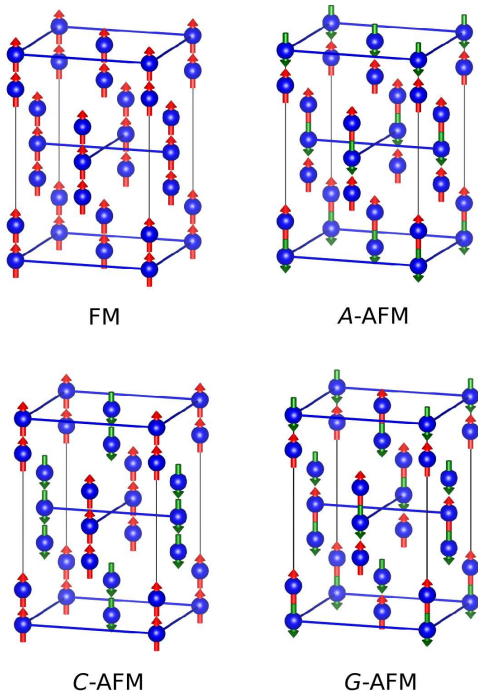
FIG. 10. AFM Ni-ion moment configurations without stripes in \text{La}_4\text{Ni}_3\text{O}_8 , F4/mmm setting. A-AFM : FM intra-trilayer, AFM inter-trilayer. C-AFM : AFM intra-trilayer, FM inter-trilayer. G-AFM : AFM intra-trilayer, AFM inter-trilayer.
