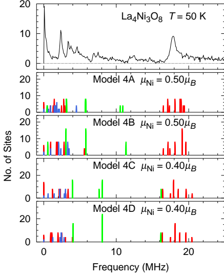
FIG. 23. Histograms of dipolar-field \mu^+ frequencies from AFM stripe Models 4A–4D compared to 50-K \mu SR FT spectrum in \text{La}_4\text{Ni}_3\text{O}_8 . Colors as in Fig. 9.
