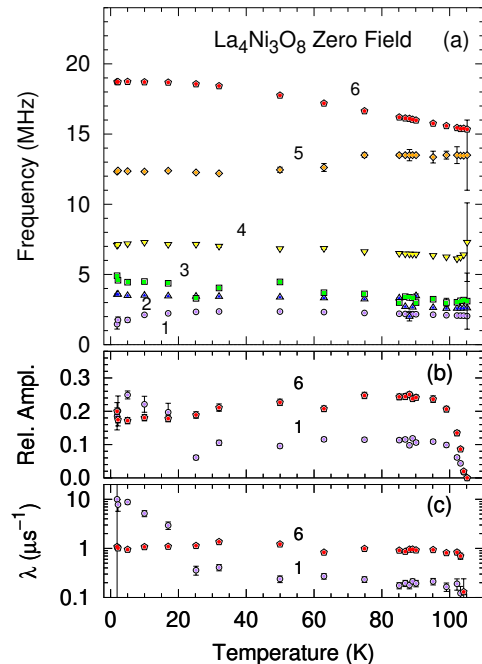
FIG. 6. Temperature dependence of parameters in \text{La}_4\text{Ni}_3\text{O}_8 from fits of Eq. (1) to ZF- \mu\text{SR} asymmetry data (cf. Fig. 5). Numbers indicate peaks in Fig. 4. (a) \mu^+ precession frequencies. (b) Relative oscillation amplitudes of Peaks 1 and 6 (Fig. 4). (c) Exponential damping rates of Peaks 1 and 6.
