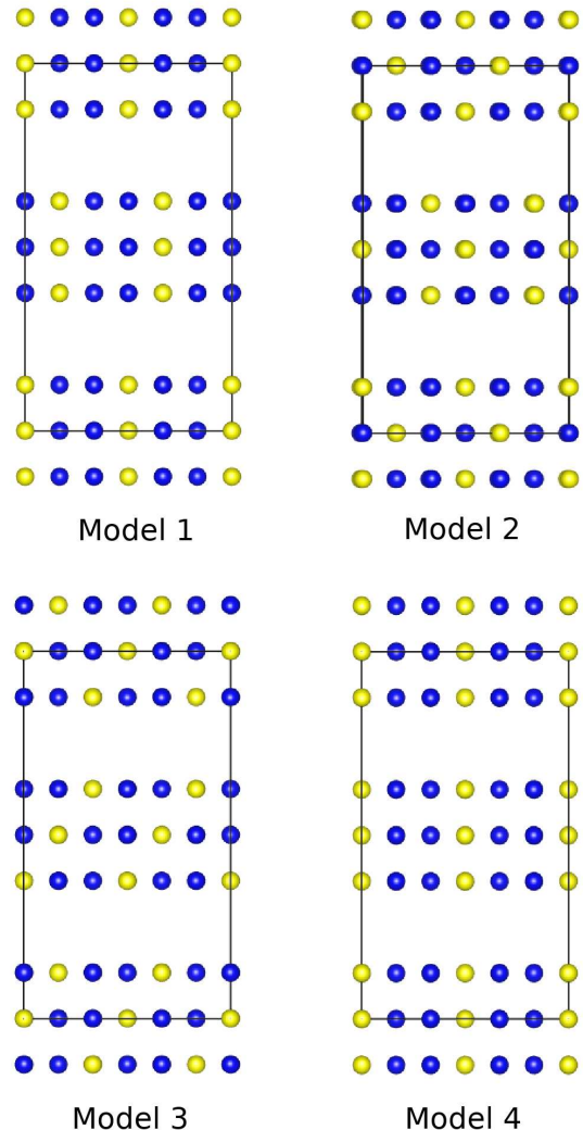
FIG. 7. Models for charge stripes in \text{La}_4\text{Ni}_3\text{O}_8 . Numbering as in Ref. 5. Blue spheres: \text{Ni}^{1+} ions ( S = 1/2 ). Yellow spheres: \text{Ni}^{2+} ions ( S = 0 ). Rectangles: 3\sqrt{2}a \times \sqrt{2}a \times c supercell outlines. The view is along the stripe ( b ) direction.
