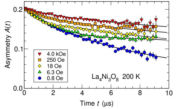
FIG. 14. Representative longitudinal-field \mu\text{SR} asymmetry relaxation in \text{La}_4\text{Ni}_3\text{O}_8 , T = 200 K. Legend: values of the longitudinal field H_L . Curves: fits of Eqs. (3)–(4) to the data.
