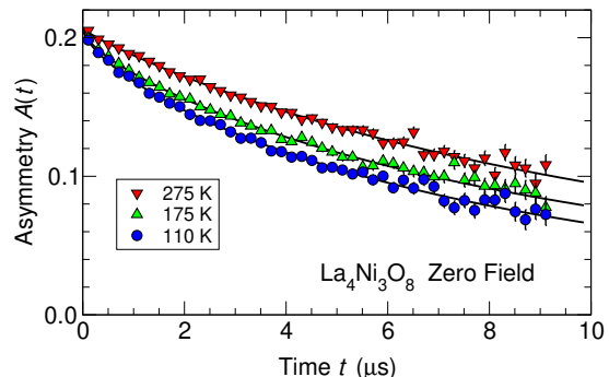
FIG. 12. Representative zero-field \mu SR asymmetry relaxation in \text{La}_4\text{Ni}_3\text{O}_8 , T > T_N . Legend: temperature values. Curves: fits of Eqs. (3) and (5) to the data.
