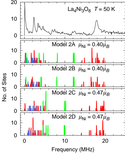
FIG. 19. Histograms of dipolar-field \mu^+ frequencies from AFM stripe Models 2A–2D compared to 50-K \mu SR FT spectrum in \text{La}_4\text{Ni}_3\text{O}_8 . Colors as in Fig. 9.
