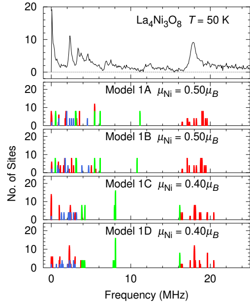
FIG. 9. Histograms of dipolar-field \mu^+ frequencies from AFM stripe Models 1A–1D compared to 50-K \mu\text{SR} FT spectrum in \text{La}_4\text{Ni}_3\text{O}_8 , T = 50 K. Colors indicate \mu^+ site groups (Table I): Red: \mu 1 – \mu 3 . Green: \mu 4 – \mu 5 . Blue: \mu 6 – \mu 8 .
