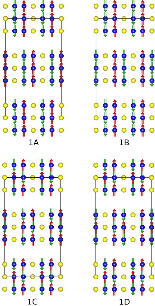
FIG. 8. AFM moment Configurations A–D in \text{La}_4\text{Ni}_3\text{O}_8 on charge stripe Model 1 [5]. Blue spheres: \text{Ni}^{1+} ions ( S = 1/2 ). Yellow spheres: \text{Ni}^{2+} ions ( S = 0 ). Rectangles: 3\sqrt{2}a \times \sqrt{2}a \times c supercell outlines. Arrows: AFM ordered moments. The view is along the stripe ( b ) direction.
