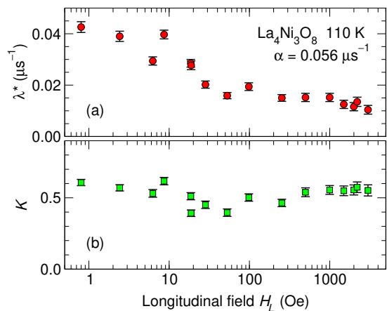
FIG. 17. Field dependence of Longitudinal-field dynamic relaxation parameters in \text{La}_4\text{Ni}_3\text{O}_8 , T = 110 K. (a) Stretched-exponential relaxation rate \lambda^* . (b) Stretching power K .
