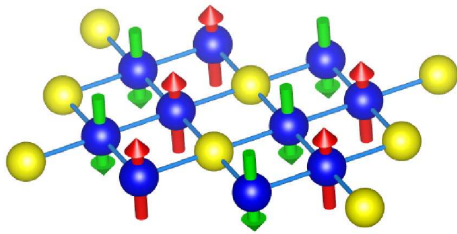
FIG. 1. Charge stripe [5] and proposed AFM moment configurations [23] on a nickel layer in \text{La}_4\text{Ni}_3\text{O}_8 . Blue spheres: \text{Ni}^{1+} ions ( S = 1/2 ). Yellow spheres: \text{Ni}^{2+} ions ( S = 0 ). Arrows: AFM ordered moments. \text{O}^{2-} ions are not shown.
