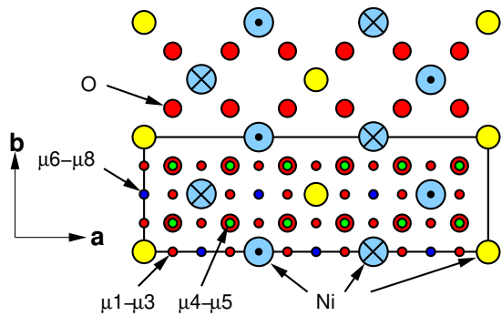
FIG. 3. 2D AFM structure of Fig. 1 [23] and projections of candidate \mu^+ stopping sites in La_4Ni_3O_8 (Fig. 2 and Table I) onto the ab plane in the F4/mmm setting of the 3\sqrt{2}a \times \sqrt{2}a 2D stripe supercell. Large circles: Blue: Ni^{1+} ( S = 1/2 ) ( \odot = up-spins, \otimes = down-spins). Yellow: Ni^{2+} ( S = 0 ). Red: O^{2-} . Small circles: \mu^+ sites from Table I. Rectangle: supercell boundary.
