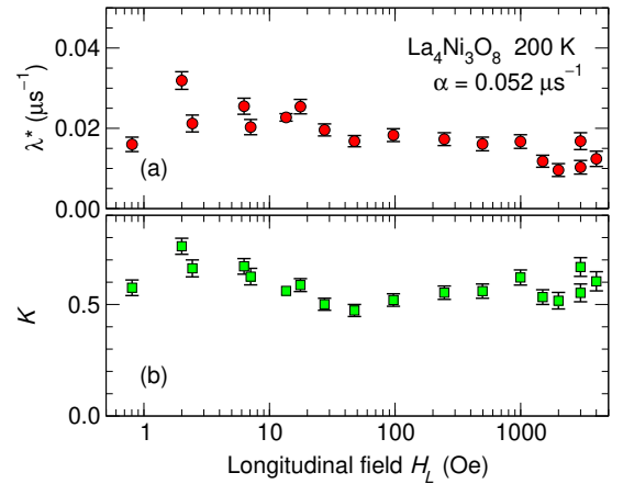
FIG. 15. Field dependence of Longitudinal-field dynamic relaxation parameters in \text{La}_4\text{Ni}_3\text{O}_8 , T = 200 K. (a) Stretched-exponential relaxation rate \lambda^* . (b) Stretching power K .
