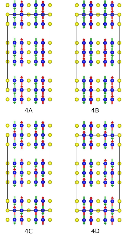
FIG. 22. AFM moment Configurations A–D in \text{La}_4\text{Ni}_3\text{O}_8 on stripe Model 4 [5]. See Fig. 8 for designations.
