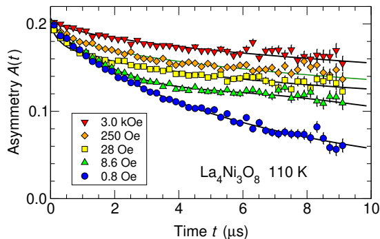
FIG. 16. Representative longitudinal-field \mu SR asymmetry relaxation in \text{La}_4\text{Ni}_3\text{O}_8 , T = 110 K. Legend: values of the longitudinal field H_L . Curves: fits of Eqs. (3)–(4) to the data.
