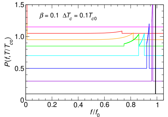
FIG. 25. Representative zero-field frequency spectra from a uniform distribution of second-order magnetic phase transition temperatures. Spectra are normalized by 0.01 for display, and are offset so that each baseline is at the corresponding temperature T/T_{c0} on the P axis. For T > T_c^{\min} spectral weight is transferred from nonzero frequencies to f = 0 .
