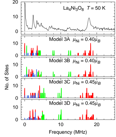
FIG. 21. Histograms of dipolar-field \mu^+ frequencies from AFM stripe Models 3A–3D compared to 50-K \mu SR FT spectrum in \text{La}_4\text{Ni}_3\text{O}_8 . Colors as in Fig. 9.
