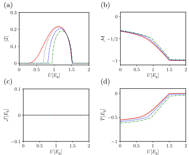
FIG. 1. (Color online) Panel (a) The excitonic order parameter |\mathcal{I}| is plotted as a function of U (in units of E_g ). Numerical results have been obtained by setting t = 0.5 E_g and \hbar\omega_c = E_g . Different curves correspond to different values of \tilde{t} . Red solid line: \tilde{t} = 10^{-4} E_g . Black dotted line: \tilde{t} = 0.05 E_g . Blue dashed line: \tilde{t} = 0.1 E_g . Green dash-dotted line: \tilde{t} = 0.15 E_g . Note that for \tilde{t} \neq 0 , |\mathcal{I}| \neq 0 for U_{c1} < U < U_{c2} . Panel (b) Same as in panel (a) but for the electronic polarization \mathcal{M} . Panel (c) Same as in other panels but for \mathcal{J} . Note that \mathcal{J} = 0 for all values of \tilde{t} and U/E_g . This implies \bar{\beta} = 0 and therefore no photon condensation. Panel (d) Same as in other panels but for \mathcal{T} (in units of E_g ).
