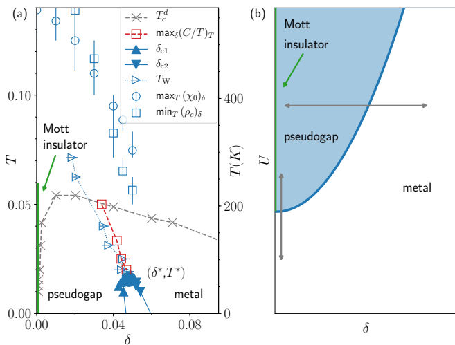
FIG. 1. Normal-state phase diagram of the two-dimensional Hubbard model within plaquette CDMFT. (a) Temperature versus doping phase diagram for U = 6.2t > U_{\text{MIT}} 14,17,29,30 . At zero doping there is a Mott insulator. At finite doping there is a first-order transition between a pseudogap phase and a metal. This first-order transition is bounded by the spinodal lines \delta_{c1} and \delta_{c2} and terminates at the critical endpoint (\delta^*, T^*) . From the endpoint emerges the Widom line, T_W , here defined as the locus of the maxima of isothermal charge compressibility \kappa_T as a function of doping 14 . The red squares indicate the loci of the maximum in specific heat as a function of doping at constant temperature. This is one of our key findings. The open circles and squares denote extrema in, respectively, spin susceptibility (from Ref. 14 ) and c -axis resistivity (from Ref. 29 ). Only below \delta^* , does the Widom line have a high-temperature precursor, where spin susceptibility drops vs T and c -axis resistivity rises vs T 29 . These indicators are often used to mark the pseudogap temperature T^*(\delta) . Crosses indicate the dynamical mean-field superconducting transition temperature T_c^d (from Ref. 31 ). On the right vertical axis we convert into physical units by using t = 350\text{meV} . (b) Sketch of the interaction strength versus doping phase diagram at low temperature. The blue line indicates the first-order transition extending from \delta = 0 17 . At \delta = 0 , for increasing U it separates a metal from a Mott insulator (vertical green line). The shaded blue region is the pseudogap, which is an emergent phase that occurs in the doped Mott insulator. Horizontal (vertical) double arrow denotes the doping-driven (interaction-driven) Mott transition.
