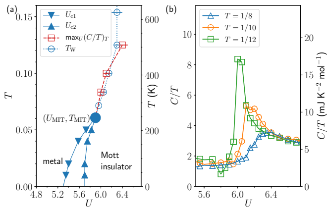
FIG. 3. (a) Temperature versus interaction strength normal-state phase diagram of the two-dimensional Hubbard model at half filling ( \delta = 0 ) within plaquette CDMFT 50 . The first-order transition between a metal and a Mott insulator is bounded by the spinodal lines U_{c1} and U_{c2} , and ends at the Mott endpoint ( U_{MIT}, T_{MIT} ). The Widom line T_W is estimated from the inflection point in the double occupancy D(U)_T (from Ref. 50 ). (b) C/T = (\partial A/\partial T)/T versus U for different temperatures. We perform numerical derivatives by finite differences between two temperatures. C/T at T = 1/8, 1/10, 1/12 is evaluated by taking finite difference between T = 1/8 and T = 1/10 , between T = 1/10 and T = 1/12 , and between T = 1/12 and T = 1/14 , respectively. Maximum of C/T as a function of U at each temperature is shown in (a) with red squares. On the right vertical axes we convert into physical units by using t = 350\text{meV} .
