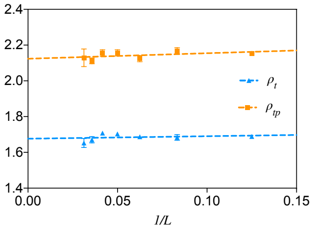
FIG. 6. Finite-size scaling of \rho_t and \rho_{tp} as a function of the inverse system size 1/L . The chemical potential is fixed at \mu = 28 for all data points such that the system is in the SF phase. Other Hamiltonian parameters are identical to Fig. 5.
