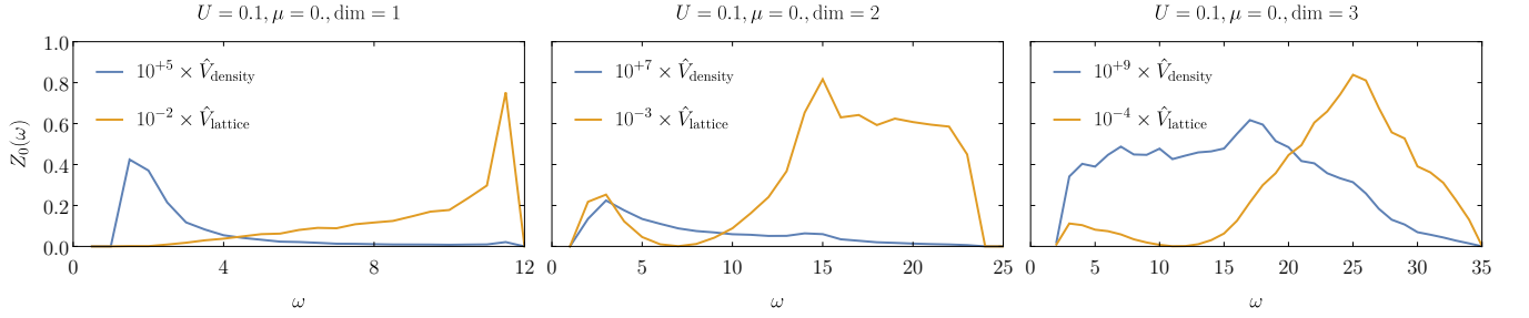
FIG. 6. Comparison: Density variation (20) and lattice modulation (21) at k = 0 . We compare the response functions from density variation with the one from lattice modulations. The response to the lattice modulation is by several orders of magnitude stronger. Note that we rescaled the data by factors of 10^{\pm x} to fit into the same range. The computations were performed for N = (501, 101^2, 41^3) for \text{dim} = (1, 2, 3) respectively. To extract a continuous response functions, we performed a binning in energy intervals of \Delta\omega = (0.5, 1, 1) for \text{dim} = (1, 2, 3) respectively.
