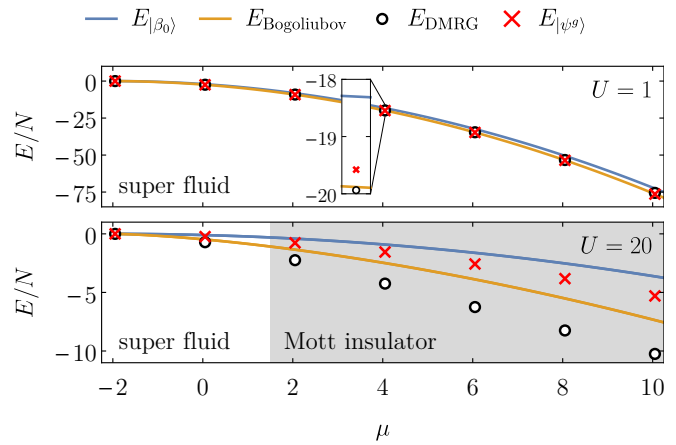
FIG. 1. Comparison of ground state energies in 1d. We compare the following approaches: (a) Minimal energy on manifold of coherent states E_{|\beta_0\rangle} from (A5), (b) Bogoliubov ground state energy E_{\text{Bogoliubov}} = E_{|\beta_0\rangle} - \Delta from (A17) in the limit N \rightarrow \infty , (c) DMRG energy E_{\text{DMRG}} and (d) minimal energy E_{|\psi_g\rangle} of all Gaussian states for N = 501 . The DMRG results were computed for finite systems with open boundary conditions and then extrapolated to the thermodynamic limit N \rightarrow \infty . The Gaussian state energy E_{|\psi_g\rangle} at N = 501 appears to have already substantially reached the thermodynamic limit value.
