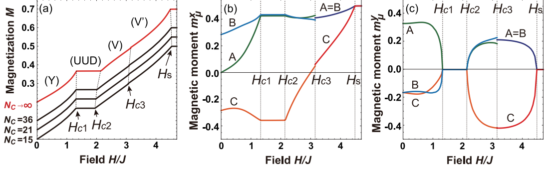
FIG. 6: (a) Theoretically simulated ground-state magnetization curves for N_C = 15, 21, 36, and \infty (from bottom to top) when H \parallel ab . The curves apart from the bottom one are vertically shifted by 0.05, 0.1, and 0.2, respectively, for clarity. (b-c) Sublattice magnetic moments \mathbf{m}_\mu ( \mu = A, B, C ) calculated by CMF+S ( \lambda \rightarrow 1 ) when H \parallel ab . The field-perpendicular components m_\mu^z are zero. The values of \mathbf{m}_\mu for \mu = A', B', C' are obtained through the relations with A, B, C as displayed in Fig. 1.
