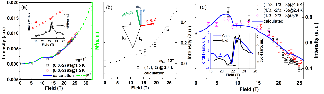
FIG. 4: (Color online) Measured (square and circle symbols) and calculated (solid lines) magnetic intensities as a function of magnetic field for the transitions between the 120^\circ -, UUD-, V- and V'-phases. (a) The magnetic contribution to the intensity of (0, 0, -2) as a function of field. Two experimental datasets (#1 and #2) are shown. The theoretical calculation (solid blue) and square of magnetization (dashed green, refer to right axis) are also presented. The inset displays the dataset #2 and its first derivative across the phase transition at 22.5 T. (b) Experimental and theoretical curves of the magnetic contribution to (-1, 1, -2) as a function of field. The inset shows a sketch of the experiment geometry. (c) The field dependence of the intensity of the (\frac{1}{3}, -\frac{2}{3}, -3) and (-\frac{2}{3}, \frac{1}{3}, -3) reflections. The inset visualizes a first derivative of the averaged experimental and theoretical datasets across the phase transition at 22.5 T. For all the datasets, the results have been scaled by a constant to allow the comparison between the experiment and the theory.
