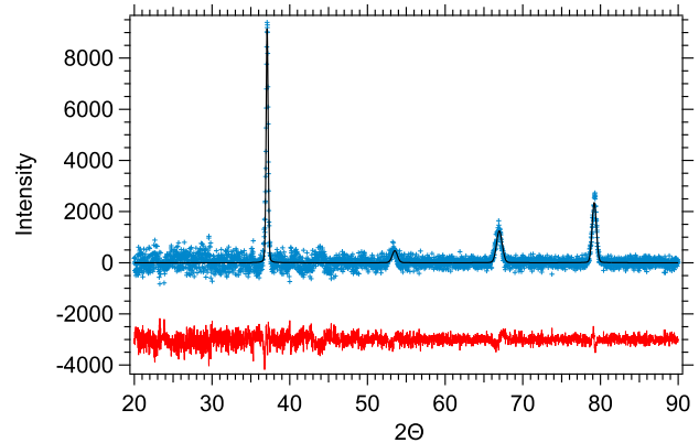
FIG. 5. Background-subtracted x-ray diffraction pattern (blue markers), fit (black line), and difference (red line, offset by -3000) for \gamma -UMo. Each peak is satisfactorily fit with the BCC structure.
