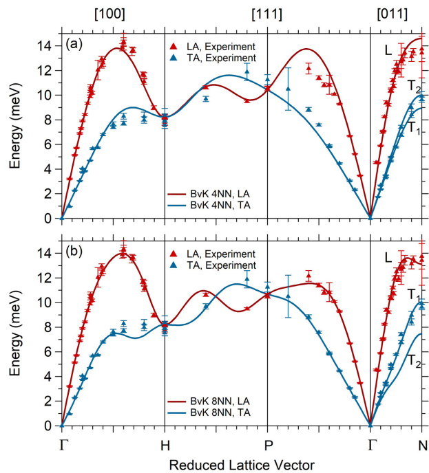
FIG. 7. Calculated dispersion curves via BvK analysis using (a) 4NN and (b) 8NN. Major differences are seen in the zone boundary modes between H and P where the data are more sparse and provide fewer constraints.
