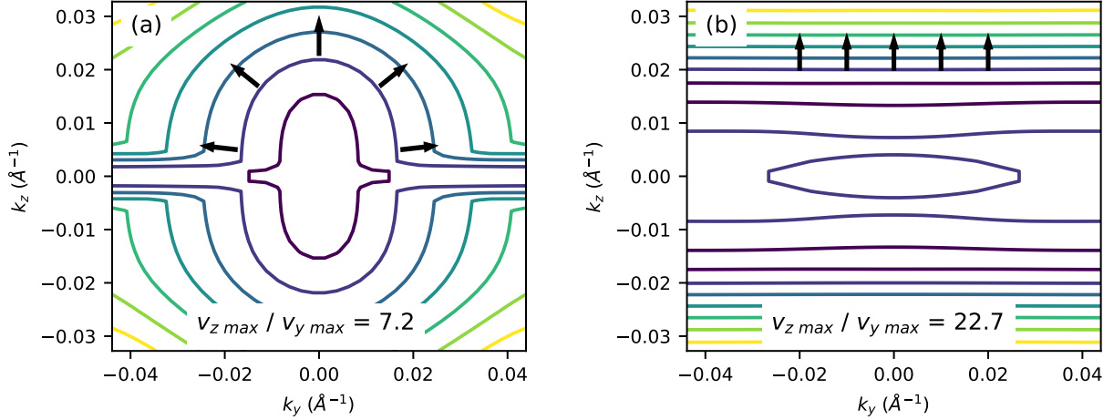
FIG. 4. Isoenergy contours in PT. (a) The isoenergy contours of an acoustic branch with an anisotropy in the maximum group velocity ratio of 7.2 in PT for the k_x = 0 plane. The lines are contours of equal frequency. The arrows show the direction of the group velocity vector. The contours are similar to those Ref. [20] corresponding to the quasi-transverse acoustic branch. (b) The isoenergy contours of an optical branch with a much larger anisotropy ratio of 22.7. The group velocity of nearly all the modes are pointed along the chain axis. We observe a similar effect in other planes in the Brillouin zone for this branch, and for other optical branches with a large anisotropy ratio.
