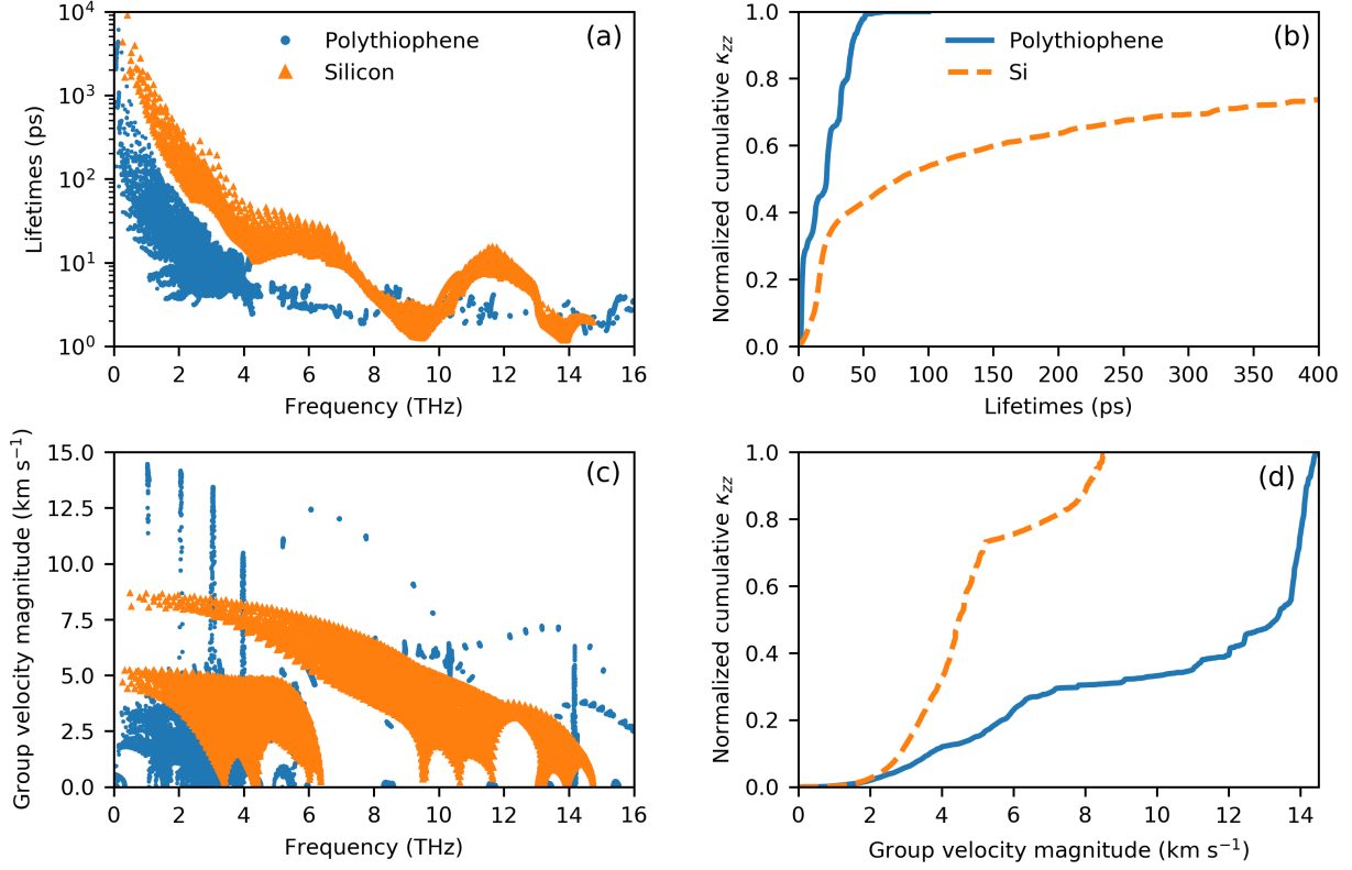
FIG. 3. Phonon lifetimes and group velocities of PT and Si. (a) Phonon lifetimes versus frequency for PT (blue dots) and Si (orange triangles). (b) Thermal conductivity accumulation function versus lifetime. The thermal conductivity of PT is due almost entirely to modes with lifetimes less than 50 ps, in contrast to Si which has more than half of its thermal conductivity from modes with lifetimes longer than 100 ps. (c) Phonon group velocities along the chain axis ( z ) versus frequency of PT (blue dots) and Si (orange triangles). (d) Thermal conductivity accumulation function versus group velocity along the chain axis. Nearly two-thirds of the heat in PT is carried by modes with group velocity larger than the maximum group velocity in Si.
