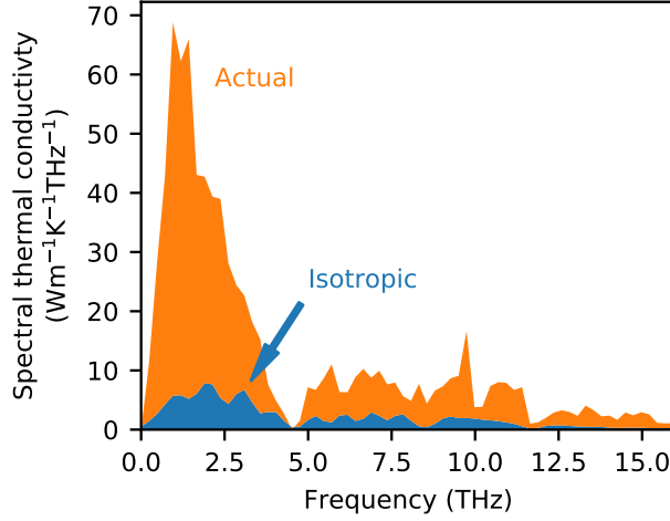
FIG. 5. The spectral thermal conductivity versus frequency in the case where the group velocities are parallel to their wave vector (blue) compared to the actual (orange). Phonon focusing underlies the high thermal conductivity of PT, particularly for modes below 5 THz.
