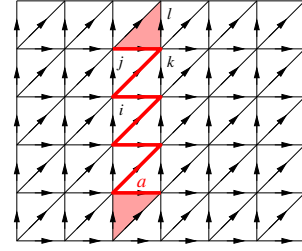
FIG. 13. (Color online) A 1-cochain a has a value 1 on the red links: a_{ik} = a_{jk} = 1 and a value 0 on other links: a_{ij} = a_{kl} = 0 . da is non-zero on the shaded triangles: (da)_{jkl} = a_{jk} + a_{kl} - a_{jl} . For such 1-cochain, we also have a \smile a = 0 . So when viewed as a \mathbb{Z}_2 -valued cochain, \mathcal{B}_2 a \neq a \smile a \text{ mod } 2 .
