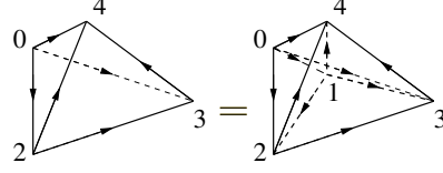
FIG. 7. A retriangulation of another 3D complex, obtained by dividing the five 3-simplices on the boundary of the 4-simplex (01234) into [(0234)] and [(0123), (0124), (0134), (1234)].
