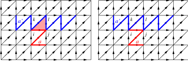
FIG. 14. (Color online) A 1-cochain a has a value 1 on the red links, Another 1-cochain a' has a value 1 on the blue links. On the left, a \smile a' is non-zero on the shade triangles: (a \smile a')_{ijl} = a_{ij}a'_{jl} = 1 . On the right, a' \smile a is zero on every triangle. Thus a \smile a' + a' \smile a is not a coboundary.
