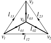
FIG. 5. The tensor C_{v_0 v_1 v_2 v_3; t_{023} t_{013} t_{123}}^{l_{01} l_{02} l_{03} l_{12} l_{13} l_{23}; t_{012}} is associated with a tetrahedron, which has a branching structure. If the vertex-0 is above the triangle-123, the tetrahedron has an orientation s_{0123} = * . If the vertex-0 is below the triangle-123, the tetrahedron has an orientation s_{0123} = 1 . The branching structure gives the vertices a local order: the i^{\text{th}} vertex has i incoming links.
