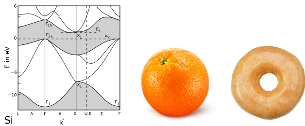
FIG. 1. “Topology” in topological insulator/superconductor (2005) corresponds to the twist in the band structure of orbitals, which is similar to the topological structure that distinguishes a sphere from a torus. This kind of topology is classical topology .
