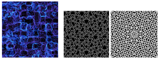
FIG. 2. “Topology” in topological order (1989) corresponds to pattern of many-body entanglement in many-body wave function \Psi(m_1, m_2, \dots, m_N) , that is robust against any local perturbations that can break any symmetry. Such robustness is the meaning of “topological” in topological order. This kind of topology is quantum topology .
