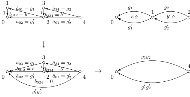
FIG. 10. Fusion of 1-morphisms.
