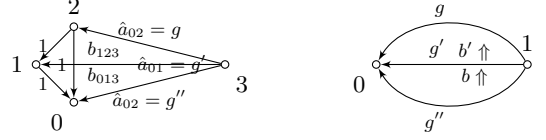
FIG. 9. The composition \cdot_v of 1-morphisms.
