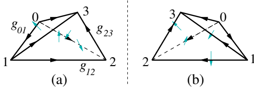
FIG. 12. (Color online) Two branched simplices with opposite orientations. (a) A branched simplex with positive orientation and (b) a branched simplex with negative orientation.
