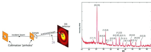
FIG. 3. X-ray scattering is a universal probe for all crystal orders.
