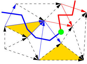
FIG. 11. A boundary configuration. The thin dash-lines corresponds to \hat{a}_{ij} = 1 . The thin colored-lines corresponds to \hat{a}_{ij} \neq 1 . The white triangles corresponds to b_{ijk} = 0 . The yellow triangles corresponds to b_{ijk} = 1 , which are boundary fermions. The non-zero \hat{a}_{ij} 's describe boundary strings on the dual lattice, represented by the thick lines. The strings with different colors are described by g and gm . The domain wall between two strings has a Majorana zero mode marked by a green dot.
