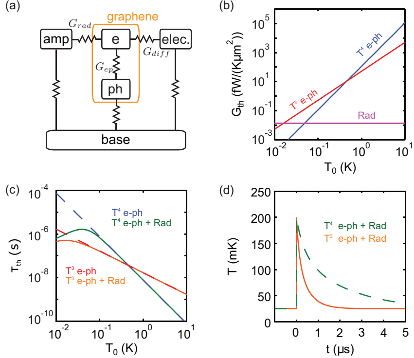
FIG. 4. (a) Thermal diagram depicting three heat transfer pathways from graphene electrons (e.) to the thermal reservoir (base) via graphene electron-phonon coupling (ph.), to the electrical contacts (elec.) via diffusion, or to the electrical environment, such as an amplifier (amp.), via photon emission (rad.). The thermal conductances in the linear response regime are denoted as G_{ep} , G_{diff} , and G_{rad} , correspondingly. (b) The thermal conductance vs. base temperature for clean graphene with a T^4 e-ph coupling law (blue), for disordered graphene with a T^3 e-ph coupling law (red), and for the radiation channel (purple). (c) The thermal time constant \tau_{th} = C_e/G_{th} in the linear response regime for clean (blue) including (excluding) radiation) and disordered (orange) including (excluding) radiation) graphene. (d) The transient thermal response of the graphene sheet upon absorbing a 26 GHz microwave photon for clean (green) and disordered (orange) graphene including radiation.
