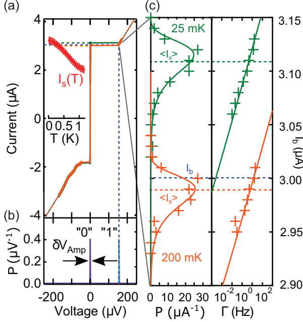
FIG. 6. (a) Measured gJj IV characteristics for electron temperature at T_0 = 25 mK (green) and T_{peak} = 200 mK (orange) with carrier density of 1.7 \times 10^{12} \text{cm}^{-2} . Inset: The measured average switching current vs. temperature. (b) The Jj voltage and the expected voltage noise from an amplifier at 1 MHz bandwidth. The blue dotted line depicts, for a given bias current in a photon event, the order of magnitude of the Jj voltage V = I_b R_n . (c) The switching probability and escape rate of the phase particle as a function of the Jj current bias. The solid line is the best fit probability distribution to the data assuming the escape mechanism is MQT. Solid lines are given by Eqn. 9 with I_c = 3.565 \mu\text{A} (25 mK) and I_c = 3.425 \mu\text{A} (200 mK).
