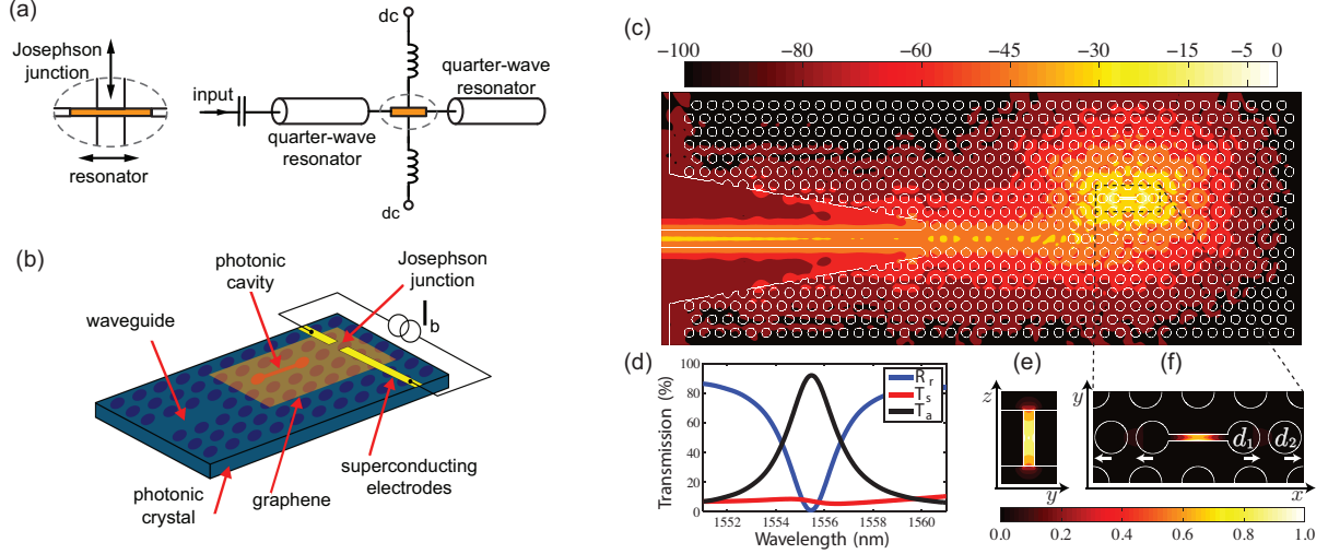
FIG. 2. Device schematic for (a) microwave and (b) infrared single photon detection. (a) The graphene flake is located at the current antinode of a halfwave microwave resonator for maximizing input efficiency. Two stages of inductors and capacitors form a high impedance network at microwave frequency for the dc measurement of the gJj. (b) A graphene sheet lies on top of a PhC cavity to increase its absorption through critical coupling. Light is coupled into the cavity through an in-chip waveguide. (c) Simulation results for critical coupling. Top view of the PhC structure overlaid with the mode profile, |\mathbf{E}|^2 , using a dB scale normalized to a maximum of 1. (d) Spectra showing the wavelength dependence of the reflection, R_r , absorption, T_a , and scattered power, T_s . (e) Cross-sectional and (f) planar view of close-ups of the cavity mode, |\mathbf{E}|^2 , using a linear scale. The parameters of the structure are: Membrane thickness, h = 250 nm, lattice period, a = 0.27\lambda , hole radius, r = 0.31a , cavity slot width, w_s = 0.032\lambda , cavity hole shifts, d_1 = 0.365a , and d_2 = 0.153a , waveguide width, w_w = 2(W\sqrt{3}a/2 - r) where W = 1.04 . The holes at the termination of the PhC waveguide are shifted along the x -axis by s_1 = 0.44a , s_2 = 0.27a , and s_3 = 0.1a .
