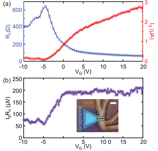
FIG. 5. (a) Measured R_n (blue) and I_s (red) as a function of V_G (b) I_s R_n versus V_G . Inset: Optical micrograph of the measured gJj whose device performance parameters were used in this report. Blue colored region is the graphene channel encapsulated by hBN and the region emphasized by orange colored lines are the NbN electrodes. Scale bar (white) is 1.5 \mu\text{m} .
