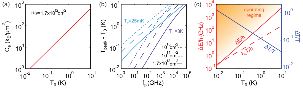
FIG. 3. (a) The specific heat of a 1\mu\text{m}^2 graphene sheet as a function of base temperature. (b) The initial temperature rise vs. frequency with electron density n_0 = 1.7 \times 10^{12} \text{ cm}^{-2} (solid, used for modeling), 10^{11} \text{ cm}^{-2} (dashed), or 10^{10} \text{ cm}^{-2} (dotted) at a base temperature of 25 mK (blue) or 3 K (purple). For an infrared detector T_0 = 3 \text{ K} will suffice but for microwave detection a lower T_0 is required to acquire a noticeable temperature change. (c) Energy resolution and temperature fluctuation of a 1 \mu\text{m}^2 graphene sheet at n_0 , representing the intrinsic noise of the calorimeter.
