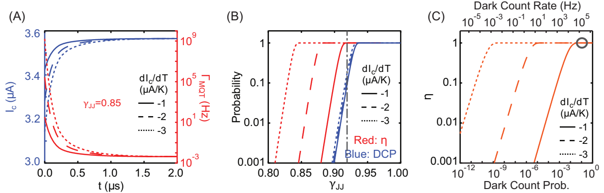
FIG. 7. (a) Change of critical current and phase slipping probability due to a single microwave photon, impinging at t = 0 s and T = 0.025 K, deduced from the graphene thermal properties and measured gJj parameters. (b) Intrinsic efficiency and dark count probability at 1 MHz count rate versus bias current. Vertical gray dashed line indicates bias current for which \eta > 0.99 for the measured dI_c/dT . (c) Trade-off between the intrinsic quantum efficiency \eta and the dark count rate at various bias currents from (b). Gray circle corresponds to gray line from (b).
