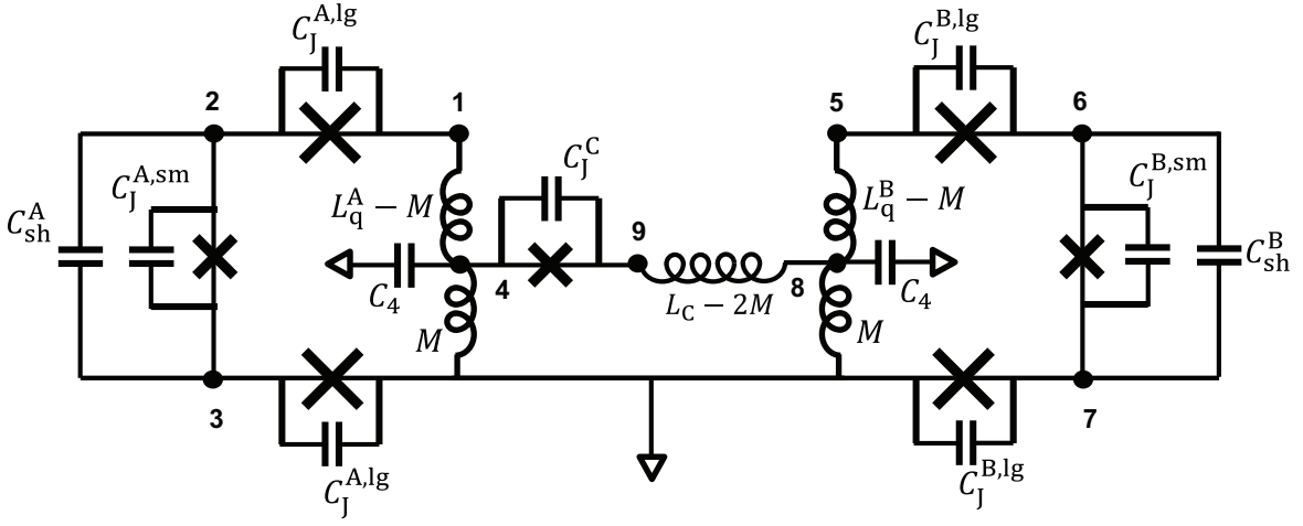
FIG. 5. Schematic diagram of the full galvanic circuit. The nodes of the circuit, labeled 1 – 9, are used to define its canonical flux and charge variables [56].
