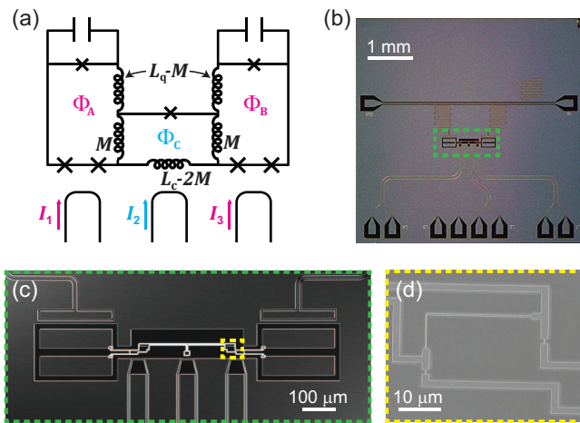
FIG. 1. Coupled qubit geometry. (a) Device schematic. Qubit A (left loop) and Qubit B (right loop) are capacitively shunted three-junction flux qubits, coupled through a shared inductance with an rf-SQUID coupler (center loop). On-chip bias currents I_1 , I_2 , and I_3 control the external fluxes \Phi_A , \Phi_C , and \Phi_B through the qubit and coupler loops. (b) Optical micrograph of the aluminum (light grey) device on a silicon (dark grey) substrate. (c) Optical image showing the qubits, coupler, and flux bias lines. (d) SEM image of the galvanic connection between Qubit B (lower-right) and the coupler (upper-left).
