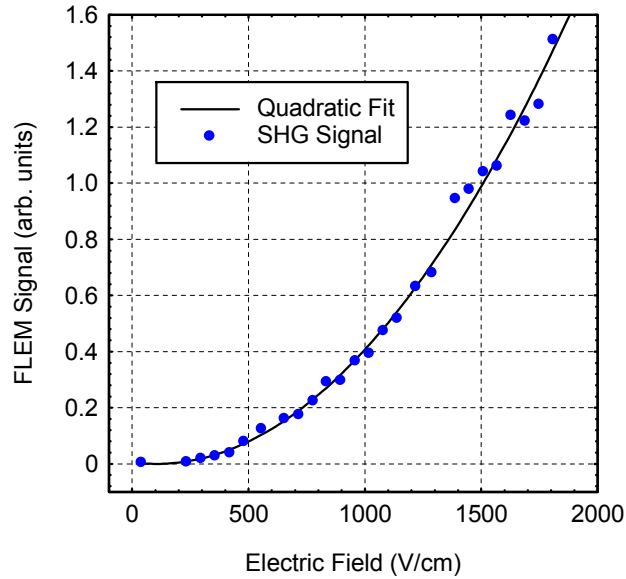
Figure 2: Quadratic fit of FLEM signal response with applied electric field. Data obtained in room air using 500 \mu\text{J} per pulse and the f = 50 cm focusing geometry.
