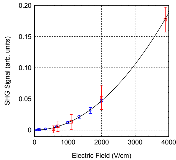
Figure 7: Quadratic dependence of SHG on the electric field applied measured while focusing the pump laser to 25 \mu\text{m} (circles), and 152 \mu\text{m} (squares), with a spatial resolution of 66 mm and 1.8 mm, respectively.
