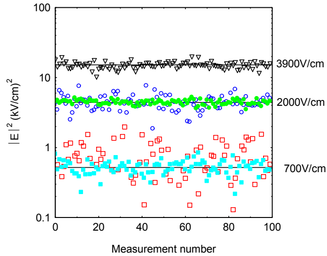
Figure 6: Signal fluctuation for E = 700\text{V/cm} (squares), 2000\text{V/cm} (circles), and 3900\text{V/cm} (triangles), while focusing to achieve a spatial resolution of 1.8 mm (open markers) and 66 mm (solid markers).
