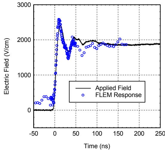
Figure 3: High voltage waveform with a voltage rise time of \sim 20 ns measured using FLEM. The FLEM calibration curve from Figure 2 was used to determine the absolute applied electric field.
