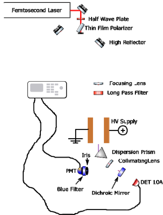
Figure 1: Femtosecond Localized E-field Measurement (FLEM) experimental setup.
