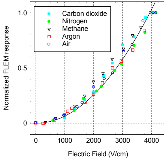
Figure 8: Normalized quadratic calibration curves for several different species. For all gases tested, second harmonic signal were readily detectable, and the standard deviation of the means did not exceed 20% of the mean values.
