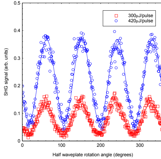
Figure 4: Second harmonic generation as a function of the half-waveplate rotation angle for 300 \mu\text{J} (red squares) and 420 \mu\text{J} (blue circles) pulses focused to a 152 \mu\text{m} spot size (FWHM) in a uniform applied electric field of 2 kV/cm.
