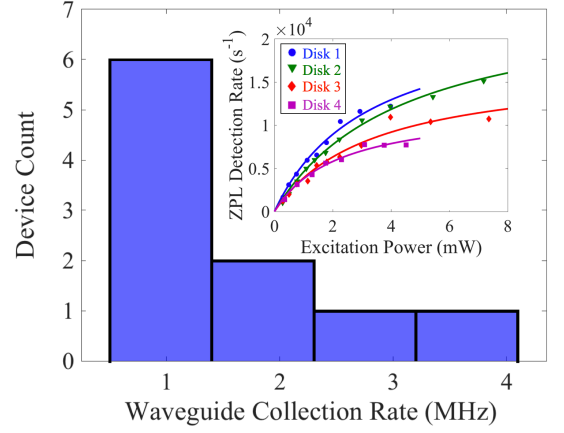
FIG. 3. Histogram of estimated saturated collection rates into bus waveguides for 10 devices. Inset: power dependence of on-resonance NV ZPL detection rate for 4 selected devices, with background removed. Solid lines are fits to saturation model.
