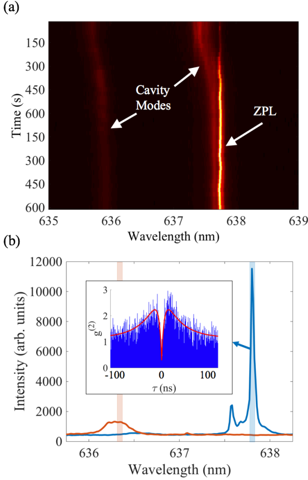
FIG. 2. (a) Measured tuning curve showing two cavity modes as one is tuned onto resonance with a coupled NV center's ZPL. (b) Grating-collected spectra with cavity tuned onto selected ZPL (blue curve) and detuned from ZPL (orange curve), with wavelength integration range used for count rate calculation indicated by shaded rectangles. Inset: photon autocorrelation measured with cavity tuned onto ZPL, with bi-exponential fit shown in red.
