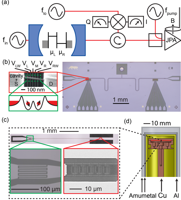
Figure 1. (a) Diagram of the experimental setup. A readout tone at frequency f_{\text{in}} is applied to the cavity input port. The output field of the cavity is sent through a circulator, amplified using a JPA and then demodulated into the I and Q quadratures. The amplification band of the JPA is flux-tuned using a small coil that creates a magnetic field B . A directional coupler is used to couple in the pump field at frequency f_{\text{pump}} . (b) Illustration of the DQD-cavity system. A single nanowire is placed on top of 5 depletion gates. Negative voltages on the gates establish a double-well potential, forming the DQD. (c) Optical micrograph of the JPA, which is implemented as a quarter-wavelength resonator shunted by an array of 5 SQUIDs. The resonator is coupled to the input port using an interdigitated planar capacitor (outlined in green). A scanning electron micrograph showing the SQUID array is outlined in red. (d) Schematic of the magnetic shielding used to isolate the JPA from the superconducting magnet around the DQD. The JPA is housed in a copper box magnetically shielded by one aluminum and two amumetal 4k cylinders.
