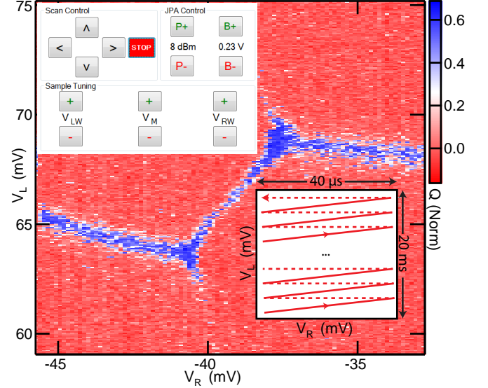
Figure 5. Normalized Q quadrature amplitude as a function of V_L and V_R . The scan was acquired by rastering the gate voltages over a 20 ms period. The rastering scheme is illustrated in the lower inset. Starting in the lower left hand corner of the stability diagram, V_R is repeatedly ramped with a 40 \mu s period. At the same time V_L is ramped up with a 20 ms period. The rastering configuration is similar to cathode-ray-tube monitors. The high SNR then allows for real-time tuning of the DQD. This is accomplished using an intuitive user interface pictured in the upper inset.
