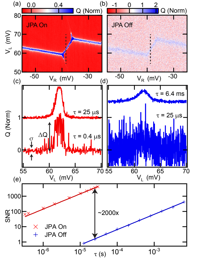
Figure 4. (a-b) Q quadrature amplitude plotted as a function of V_L and V_R near the (n, m+1) \leftrightarrow (n-1, m+2) interdot charge transition. (a) Data taken with the JPA on, and (b) with the JPA off. For both cases each point of the colormap is integrated for \tau = 42 \mu\text{s} . (c-d) Traces of the Q quadrature amplitude showing the interdot charge transition for different per-point integration times \tau . (c) Data taken with the JPA on (traces are offset by 1 for clarity), and (d) with the JPA off (traces are offset by 1.5 for clarity). (e) Signal-to-noise ratio (SNR) for the interdot charge transition as a function of the integration time \tau . Amplification with the JPA results in a factor of 2000 improvement in the SNR. Solid lines are fits to Eq. 2.
