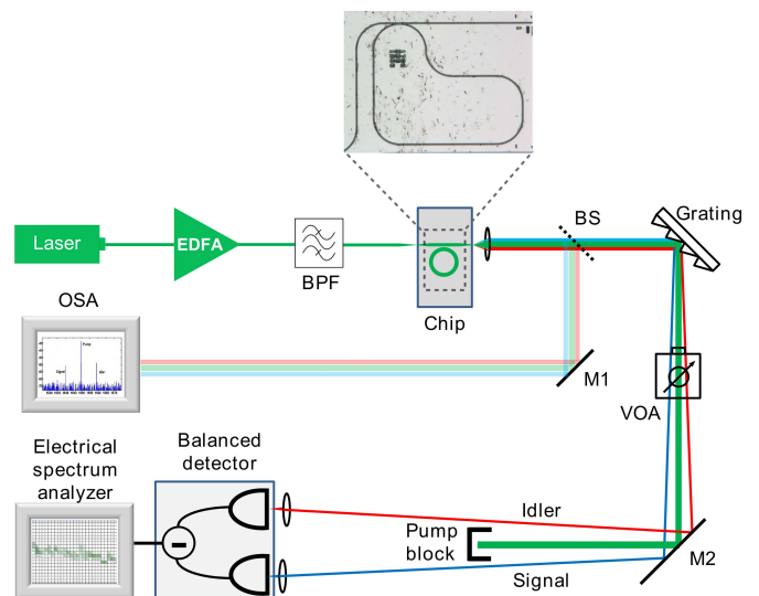
FIG. 2. Experimental setup. The on-chip microring resonator is pumped by a continuous wave laser followed by an erbium doped fiber amplifier (EDFA) from JDS Uniphase and a bandpass filter (BPF). To ensure efficient coupling in and out of the chip, inverse tapers are used [37]. A lensed fiber is used for input coupling. The output from the waveguide is collected with a high NA objective lens. The diffraction grating spatially separates the pump and the twin beams. After blocking the pump, the beams are focused on a balanced detector. The RF output of the balanced detector is sent to an electrical spectrum analyzer. A small fraction of the beams is sent to an optical spectrum analyzer (OSA) to monitor the onset of parametric oscillation. The inset shows a microscope image of the ring resonator coupled to the bus waveguide. The shape of the fabricated ring is non-circular to fit the resonator within one field of the electron beam lithography tool and hence avoid stitching errors. EDFA: Erbium doped fiber amplifier. BPF: Bandpass filter. OSA: Optical spectrum analyzer. VOA: Variable optical attenuator. M1, M2: mirrors. BS: Beam splitter
