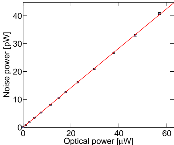
FIG. 4. Shot noise calibration, showing the linearity of the noise power in the photocurrent difference with optical power, as expected from theory. The data are taken at a Fourier sideband frequency of 3 MHz, using a spectrum analyzer with a resolution bandwidth of 30 kHz and a video bandwidth of 100 Hz. Data points have been corrected by subtracting the electronic noise of the balanced detection system. Error bars are extracted from the raw data.
