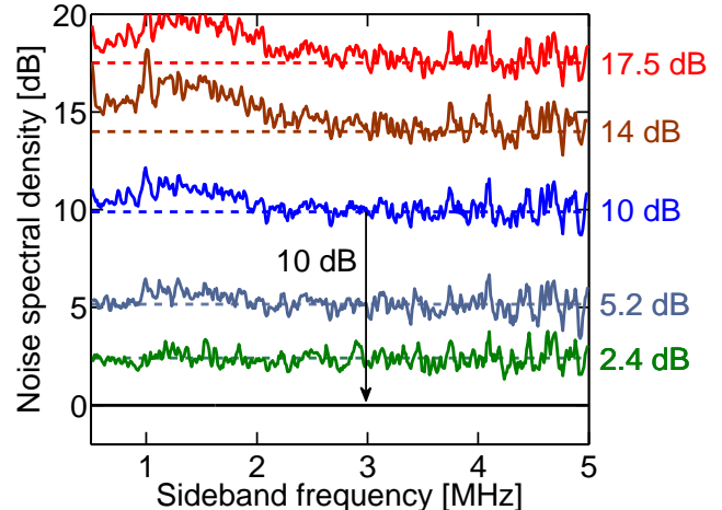
FIG. 3. Linearity of the balanced detection system from 0.5 MHz to 5 MHz. The data have been dark noise corrected and normalized to the shot noise spectrum at a base local oscillator (LO) power of P_0 = 7.8 \mu\text{W} , corresponding to the horizontal solid line at 0 dB. The dashed lines depict the mean optical power in the corresponding spectrum referenced to the base LO power P_0 , in dB. There is significant technical noise at low frequencies, which is clearly evident at relative powers above 10 dB. The data have more fluctuations at high frequencies due to higher electronic noise and consequently lower dark noise clearance for the base LO power P_0 . The dark noise varies from 5 dB below the 0 dB reference at 0.5 MHz to 1 dB below the reference at 5 MHz. Around 3 MHz, the detection system is linear over more than 20 dB, which is also substantiated by the linearity of the shot noise calibration measurement in Fig. 4.
