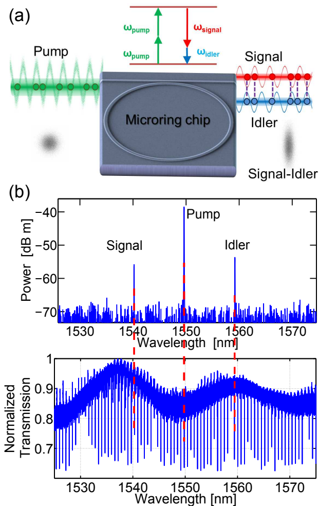
FIG. 1. (a) Schematic of the generation of intensity correlated signal and idler beams via four wave mixing in the on-chip microring optical parametric oscillator (OPO). (b) Top: Optical spectrum analyzer scan of the light coupled out of the chip, at a pump power just above the parametric oscillation threshold. The \text{Si}_3\text{N}_4 ring is pumped at 1549.6 nm, generating signal and idler modes at 1540.2 nm and 1559.2 nm, respectively, which are 15 cavity modes away from the pump wavelength, as can be seen in the bottom figure. Bottom: Transmission spectrum of the ring for transverse electric (TE) polarization.
