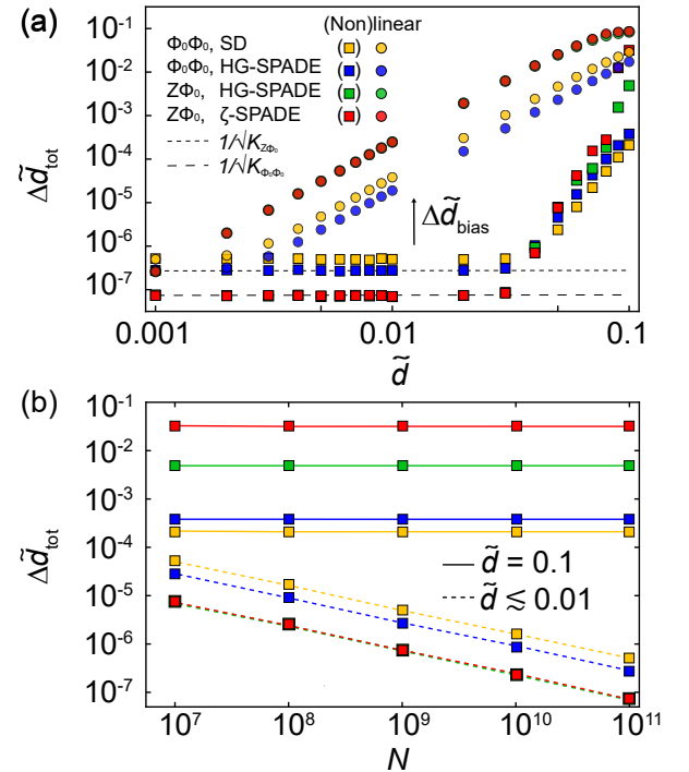
FIG. 4. (a) Simulated total measurement error versus actual displacement for various transceiver architectures, using linear and nonlinear estimators. (b) Simulated total measurement error versus photon number in the shot noise (dashed) and bias (solid) limited regime.
