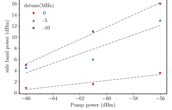
FIG. 6. Side band power as function of pump power for three different frequency detune or current bias point. In this power measurement we have deducted the noise floor of the spectrum analyzer from the peak power of the side bands.
