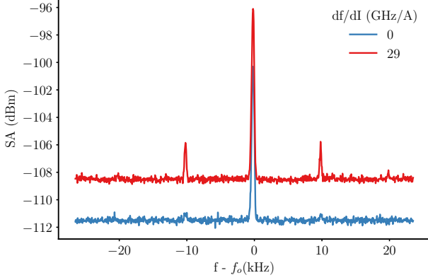
FIG. 4. Frequency upconversion of a 10kHz low frequency signal through a carrier tone at resonator frequency f_o . Without frequency detuning or current bias df/dI_{dc} = 0 minimum upconversion is observed above the noise floor of our measurement (blue curve). Applying a DC bias that shifts the resonance by 10MHz (corresponding to df/dI_{dc} \neq 0 ) we observe clear frequency upconversion as side bands around the center carrier peak (red curve).
