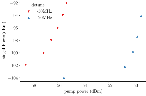
FIG. 7. Measured signal peak power under non-degenerate three-wave pumping as function of pump power at two frequency detuning points.
