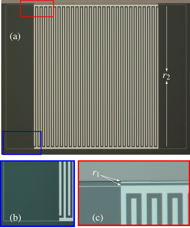
FIG. 2. a , image of the tunable resonator. Lighter color marks the Lumped LC resonator and the readout line that carries both the RF and DC signals. Darker color is the silicon substrate. In the center is the interdigitated capacitor and the narrow lines on both sides are the inductors. r_2 is the distance from the further end of the loop to the readout line that is used for flux calculation. b , zoom in image of the inductor with width of 400 nm and interdigitated capacitor in the blue rectangle of a . c , coupling of the LC resonator to the read out line corresponding to the area outlined by the red square of a . Darker color is the Nb readout line and the lighter color is part of the LC resonator. Q_c (coupling quality factor) for the resonator is determined by the gap between the resonator and the readout line, which we designed to be 2 \mu\text{m} . r_1 is the distance from the closest end of the loop to the readout line that is used for flux calculation.
