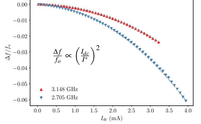
FIG. 3. Relative resonance shift \Delta f/f_o as a function of DC bias current for the two Al resonators. The resonant frequency shifts to lower values with increasing biasing current following a parabolic relationship as expected from Eq. 4. Dashed lines are fits to a quadratic equation.
