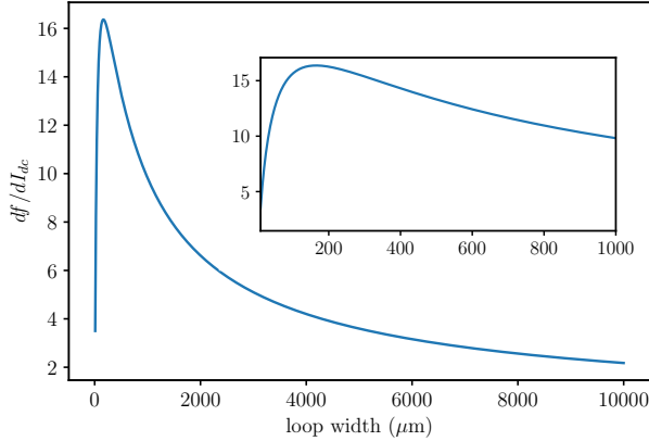
FIG. 9. \partial f/\partial I_{dc} as function of loop width W for loop strip of 1\text{ }\mu\text{m} . Maximum happens at W \approx 200\text{ }\mu\text{m} . Inset is zoom in to the range of 1000\text{ }\mu\text{m} to show the maximum point.
