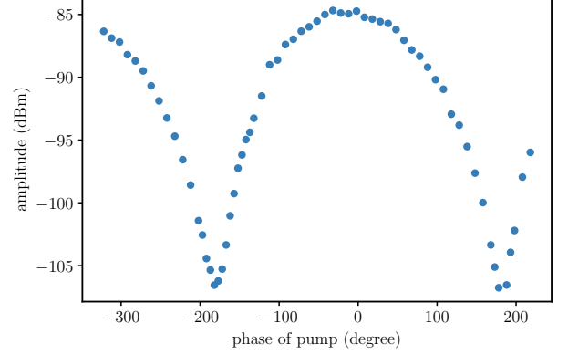
FIG. 8. Measured signal peak power under degenerate three-wave pumping as function of pump phase. Both signal power and phase as well as pump output power from generator remain constant during measurement while phase of the pump was changed by adjusting the phase parameter on the generator. Power of pump was set at -51 dBm. An arbitrary phase offset has been removed to set the phase maximum at zero.
