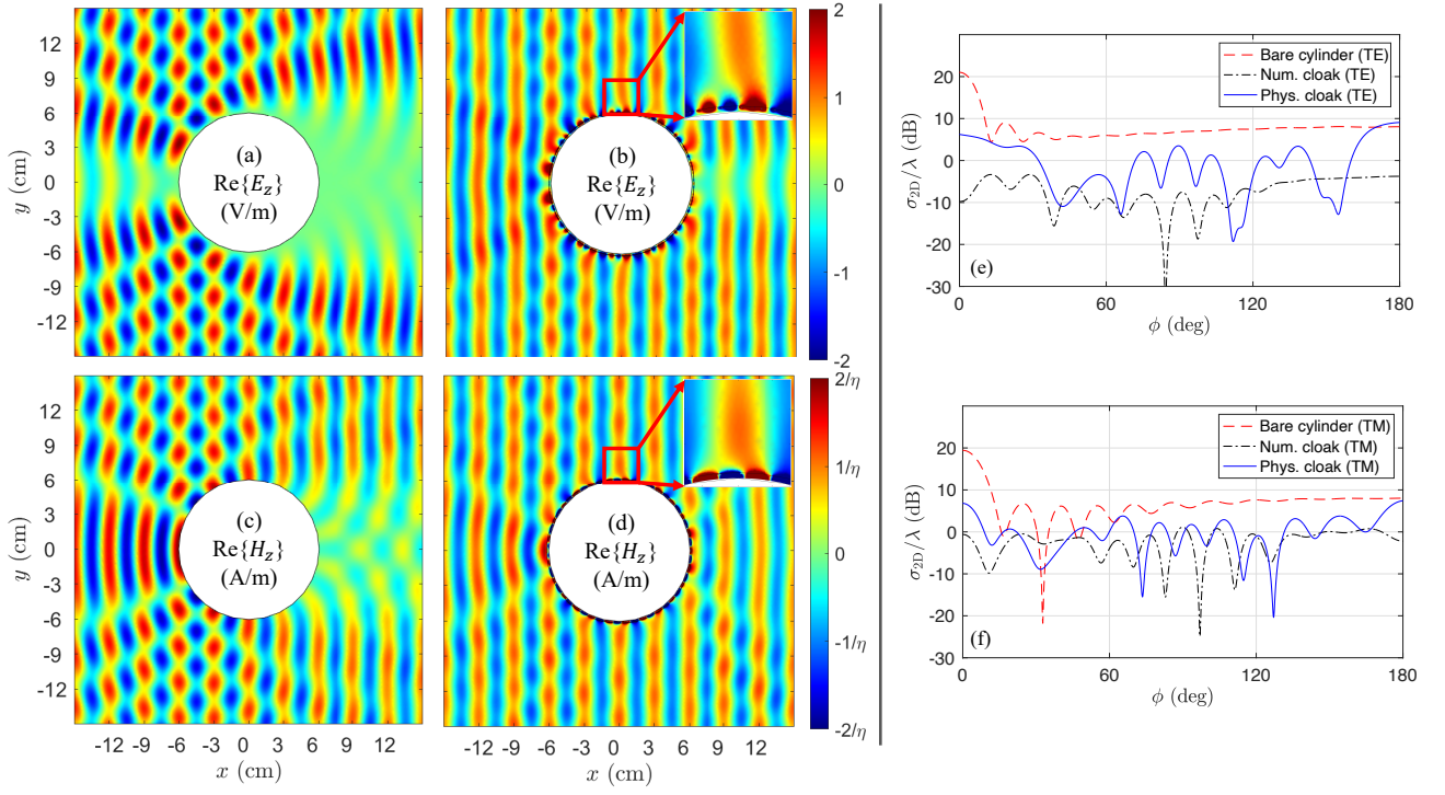
FIG. 6. 3-D simulation results for scattering scenarios with bare and cloaked 4\lambda -diameter PEC cylinders for the two polarizations. Snapshots of the total E_z(x, y) distribution for (a) the bare PEC cylinder and (b) the cloaked cylinder in TE polarization. Snapshots of the total H_z(x, y) distribution for (c) the bare PEC cylinder and (d) the cloaked cylinder in TM polarization. The insets of (b) and (d) show the magnified views of the near the topmost parts of the cloak for each polarization. Comparison of the 2-D bistatic RCS between the bare PEC cylinder, the numerical cloak, and the physical cloak in the (e) TE and (f) TM polarization.
