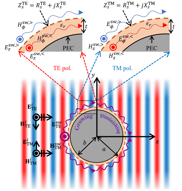
FIG. 1. A 2-D configuration of dual-polarized metasurface cloaking. An incident PW propagates in the +x -direction and illuminates the cloaked PEC cylinder. At top, a magnified view of the SWs flowing conformally along the metasurface is illustrated for each polarization.
