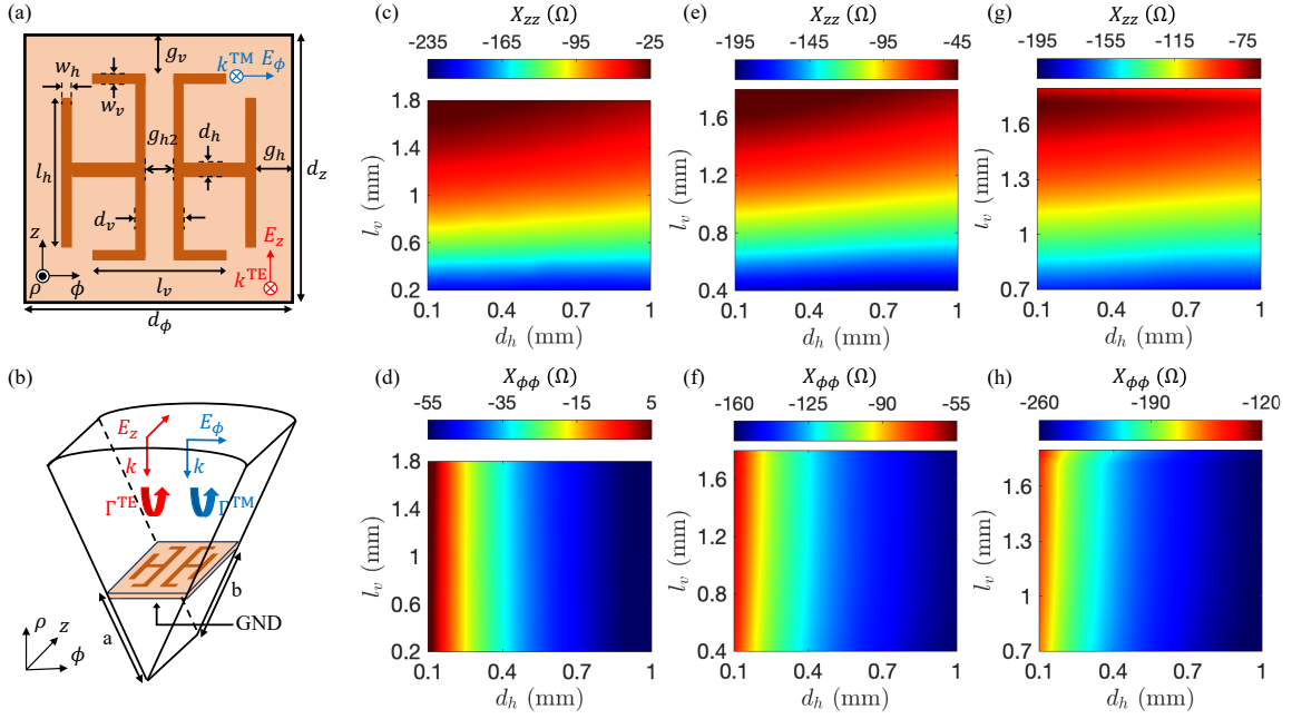
FIG. 4. Printed meta-atom design for surface reactance realization for the two polarizations. (a) Top view of a unit cell having a printed Jerusalem cross with a vertical gap in the \phi -direction. There are three design parameters: d_h , g_{h2} , and l_v . The gap g_{h2} is selected among 0, 0.1, and 0.4. Fixed dimensions are as follows: d_z = 3 , d_\phi = 3 , l_h = 1.8 , g_h = 0.05 , w_h = 0.1 , d_v = g_{h2} + 0.3 , w_v = 0.1 , g_v = 0.05 . (b) A meta-atom inside a wedged-plate cylindrical waveguide. (c) X_{zz} for g_{h2} = 0 . (d) X_{\phi\phi} for g_{h2} = 0 . (e) X_{zz} for g_{h2} = 0.1 . (f) X_{\phi\phi} for g_{h2} = 0.1 . (g) X_{zz} for g_{h2} = 0.4 . (h) X_{\phi\phi} for g_{h2} = 0.4 . Units for all lengths are millimeter.
