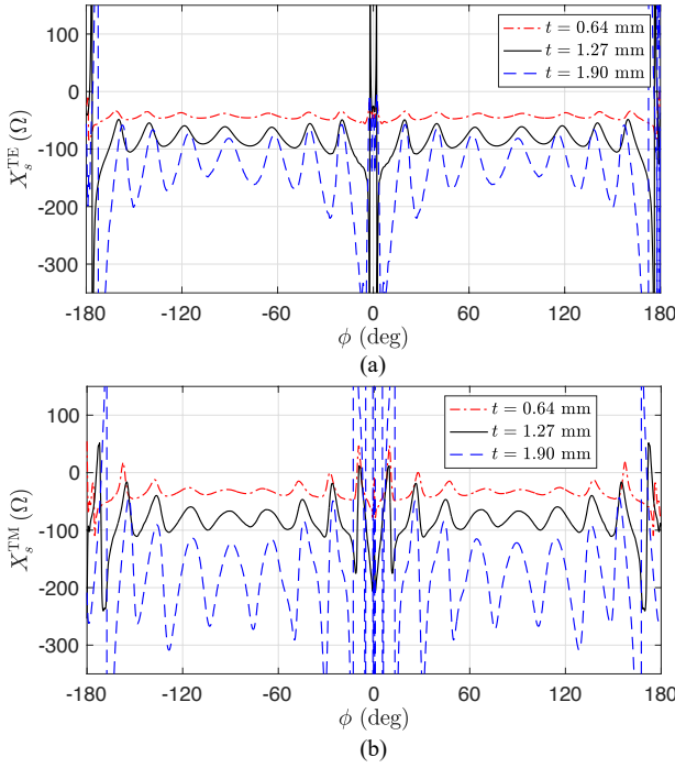
FIG. 3. Optimized distributions of X_s(\phi) for the metasurface cloak for different substrate thicknesses t = 0.64, 1.27 , and 1.9 mm, designed to conceal a conducting cylinder with a radius of 2\lambda at 10 GHz. The relative permittivity \epsilon_r of the dielectric shell is fixed at 10.2 . (a) TE polarization. (b) TM polarization.
