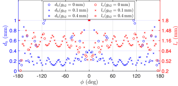
FIG. 5. Design parameters for the optimized physical metasurface design for dual-polarized cylindrical cloaking of a 2\lambda -radius cylinder.
