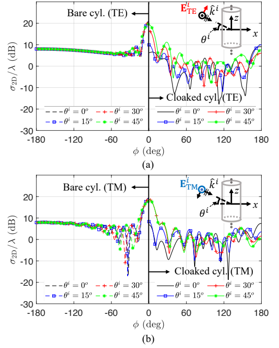
FIG. 7. Simulated 2-D bistatic RCSs of a bare cylinder and the printed metasurface cloak for incident PWs with an oblique incident angle \theta^i . (a) 2-D RCS for TE polarization (equivalent to the TM-to- z polarization). (b) 2-D RCS for TM polarization (equivalent to the TE-to- z polarization). For both polarizations, the RCSs for the bare and cloaked cylinders are plotted over \phi \in [-\pi, 0] and \phi \in [0, \pi] , respectively. The RCS in each scenario has a mirror symmetry with respect to \phi = 0 .
