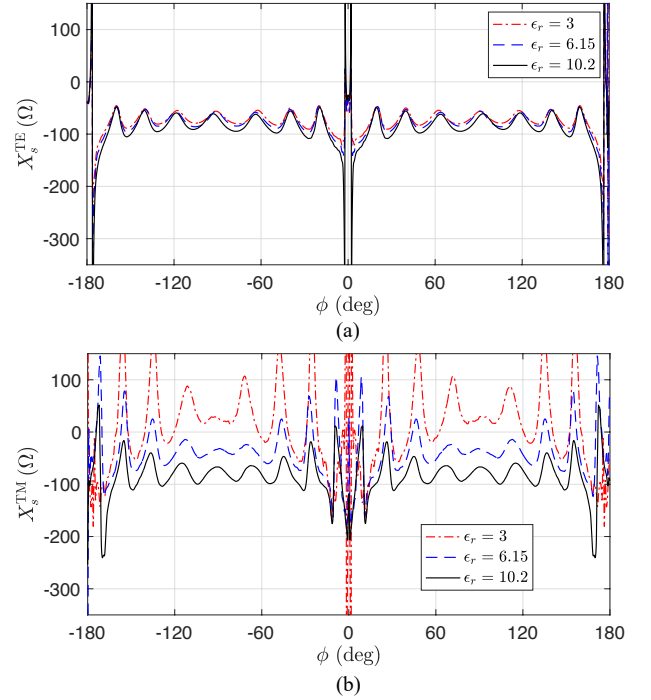
FIG. 2. Optimized distributions of X_s(\phi) for the metasurface cloak for different relative permittivities \epsilon_r = 3, 6.15 , and 10.2 , designed to conceal a conducting cylinder with a radius of 2\lambda at 10 GHz. The thickness t of the dielectric shell is fixed at 1.27 mm. (a) TE polarization. (b) TM polarization.
