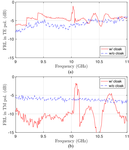
FIG. 10. Forward restoration level with respect to frequency, defined by |S_{21,\text{cloaked}}/S_{21,\text{uncloaked}}(\phi = 0)/S_{21,\text{freespace}}(\phi = 0)| in dB scale for (a) TE and (b) TM polarizations.
