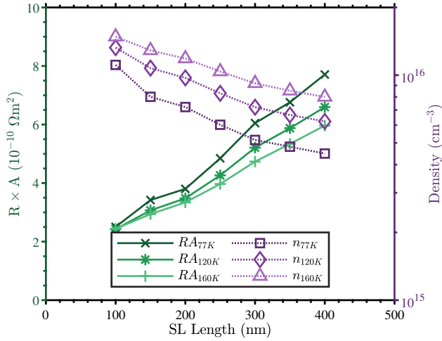
FIG. 9. The resistance-area product (green lines) and electron density (purple dotted lines), respectively, calculated for majority electrons as a function of simulation size at temperatures of 77 K, 120 K, and 160 K. Linear regression on the resistance results in R-squared values of 0.990, 0.992, and 0.993, respectively. There is strong linearity at all temperatures, but the electron density inconsistency suggests that resistance scaling using Eq. (8) will not be accurate for electrons.
