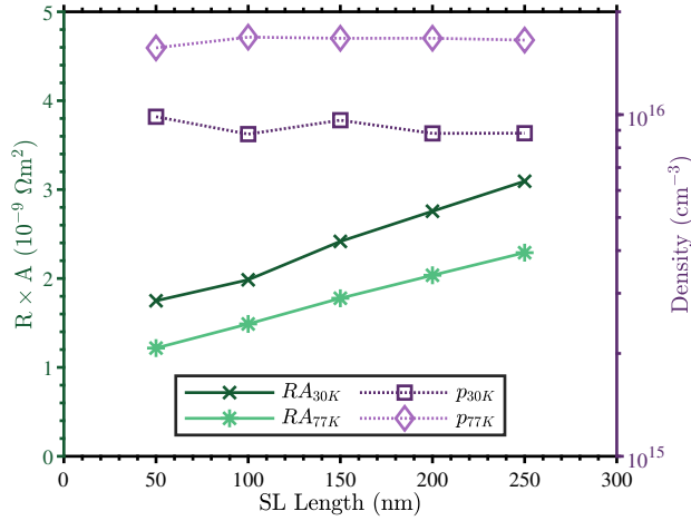
FIG. 6. The resistance-area product (green lines) and hole density (purple dotted lines), respectively, calculated for majority holes as a function of simulation size at temperatures of 30 K and 77 K. Strong linearity of resistance is demonstrated at both temperatures, but the hole density is noticeably less consistent at 30 K. Linear regression on the 30 K (77 K) resistance data gives an R-squared value of 0.994 (0.999).
