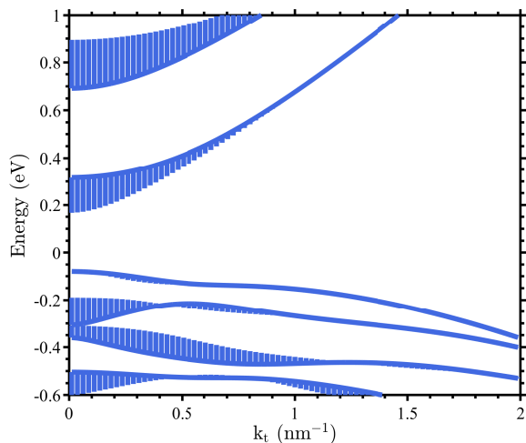
FIG. 1. The calculated energy band structure of a 3/3 nm InAs/GaSb SL plotted as a function of the transverse wave vector and modified with vertical lines representing the dispersion in the vertical wave vector. The band gap results in a cut-off wavelength of \sim 5 \mu\text{m} indicating that this is a MWIR SL structure.
