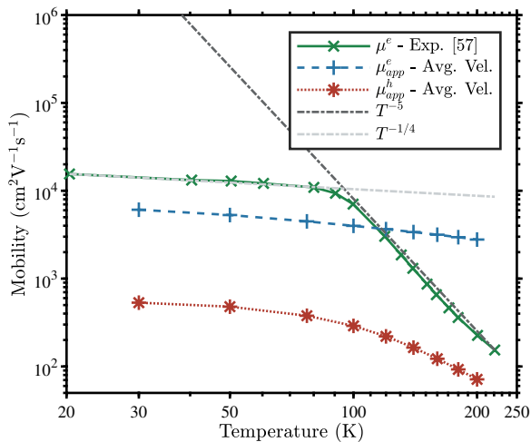
FIG. 3. The vertical electron mobility as a function of temperature (green line with x's) for a \sim 4.3 \mu\text{m} LWIR SL as reported by Swartz and Myers [57]. Also plotted are the apparent vertical electron (blue dashed line with pluses) and hole (red dotted line with asterisks) mobilities calculated using the average velocity method for a 200 nm MWIR T2SL. The experimental mobility transitions from a T^{-1/4} to a T^{-5} dependence at \sim 90 K suggesting a qualitatively similar transition between coherent and diffusive transport as with the calculated hole mobility.
