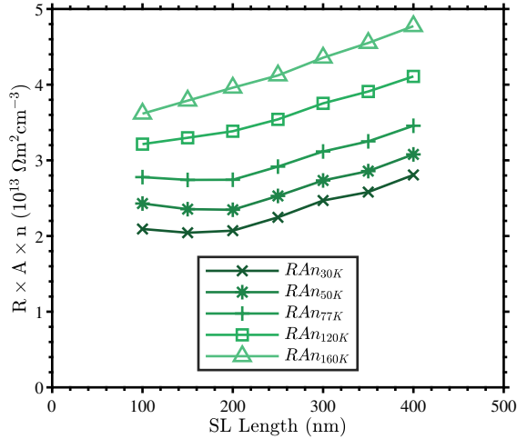
FIG. 10. The resistance-area-density product calculated for majority electrons as a function of simulation size at several temperatures. Linear regression was performed on the calculations with lengths of 200 nm and greater returning R-squared values of 0.992, 0.995, 0.997, 0.998, and 0.997, respectively, suggesting that valid mobilities may be extracted using Eq. (9).
