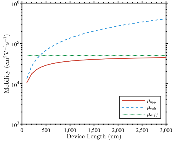
FIG. 14. The apparent, ballistic, and diffusive-limited mobilities calculated for an example InAs device at 77 K as a function of device length. It is clear that the apparent mobility for a smaller device significantly underestimates the mobility in a larger device.
