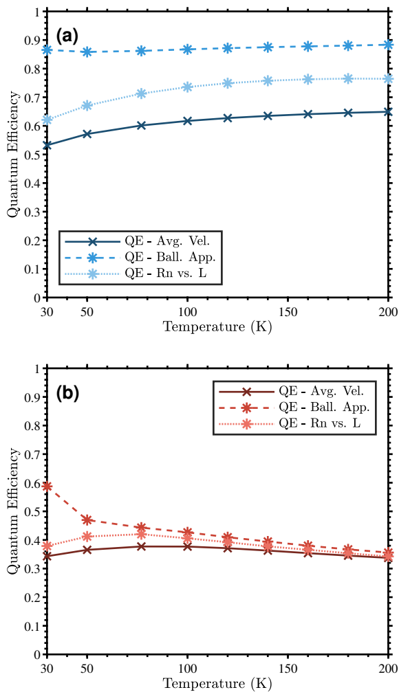
FIG. 15. The approximate quantum efficiency calculated for an electron-based (a) and hole-based (b) T2SL photodetector. The inconsistency between the QEs calculated using the different methods is commensurate with that of the mobilities, exemplifying the impact that mobility extraction methodology can have on predictions of device performance.
