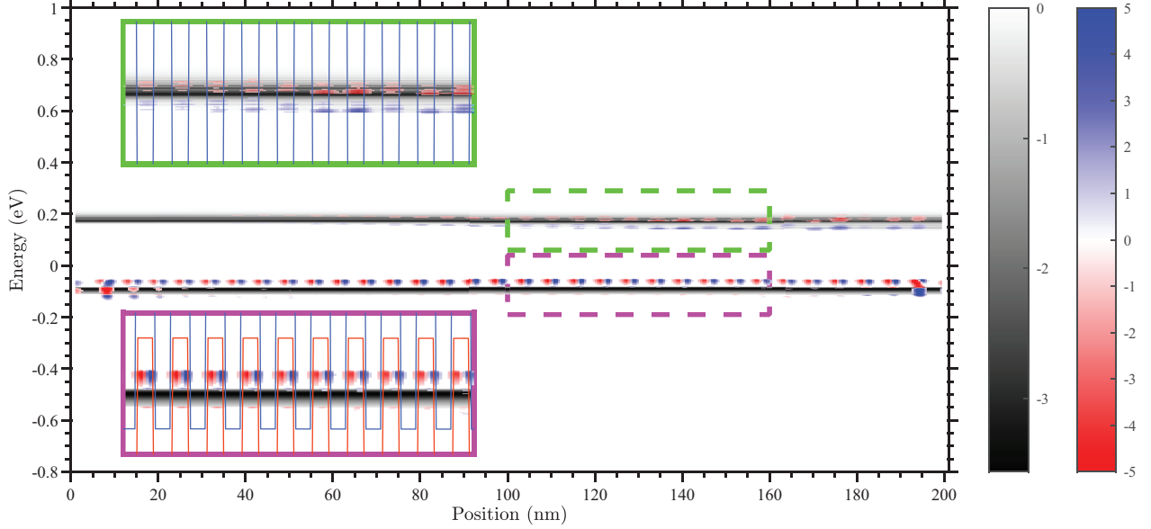
FIG. 11. The electron (data at higher energy levels) and hole (data at lower energy levels) spatially resolved spectral currents (in 10^6 \text{ Acm}^{-2} and 10^4 \text{ Acm}^{-2} , respectively) and in-scattering rates (in 10^{26} \text{ s}^{-1}\text{cm}^{-3} and 10^{24} \text{ s}^{-1}\text{cm}^{-3} , respectively) associated with POP scattering for a 200 nm simulation at 77 K. POP scattering is size-dependent for electrons, but nearly size-independent for holes at this scale. Note that this figure is a composite plot of two separate calculations, one for electrons and one for holes, with electric field strengths of 100 \text{ V cm}^{-1} and 2,000 \text{ V cm}^{-1} , respectively. Thus, the SL band diagrams were only included in the two insets as they would conflict in the composite plot. (The spectral currents are displayed in a grayscale colormap while the POP in-scattering rates are displayed in a blue/red colormap.)
