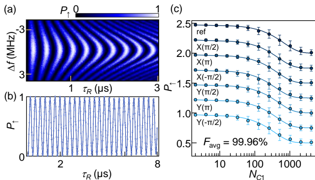
FIG. 4. Single qubit randomized benchmarking. (a) P_{\uparrow} as a function of the frequency detuning \Delta f from resonance (19.105 GHz) and \tau_R . (b) High visibility Rabi oscillations from driving the qubit on resonance. (c) Return probability P_{\uparrow} as a function of N_{C1} for each IRB curve (including the reference) showing high visibility, full saturation, and average gate fidelity 99.96%. The curves are offset by 0.25 for clarity.
