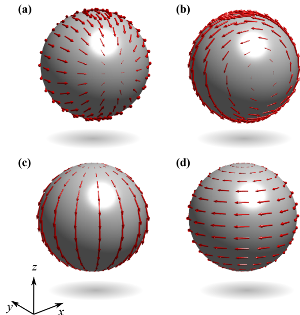
FIG. 2. (Color online) Depiction of the spin-orbit field-like and damping-like torques over the unit sphere. The conventional damping-like and field-like torques are shown panels (a) and (b), respectively. The unconventional damping-like and field-like spin-orbit torques are depicted in panels (c) and (d), respectively. These correspond to the four terms in the spin-orbit torque density in the Landau-Lifshitz-Gilbert equation, as defined in Eq. (1).
