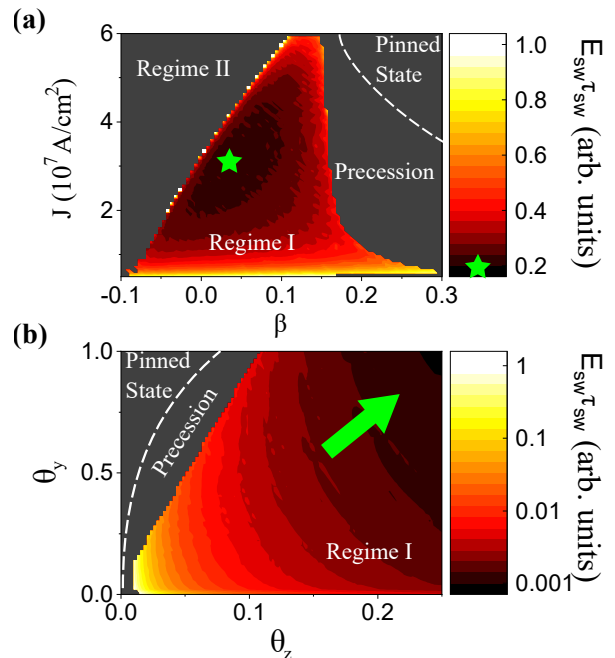
FIG. 7. (Color online) Regime I normalized switching energy-delay product, E_{\text{sw}}\tau_{\text{sw}} , of a perpendicular magnetization subjected to both CSOT and USOT. (a) Current density vs field-like to damping-like torque ratio ( J vs \beta ) diagram, at fixed \theta_y = 0.6 and \theta_z = 0.05 . The energy-delay product was normalized by that of J = 0.5 \times 10^7 \text{ A/cm}^2 and \beta = 0.15 . The green star highlights the optimal energy-delay product. (b) \theta_y vs \theta_z diagram, at fixed J = 3 \times 10^7 \text{ A/cm}^2 and \beta = +0.2 , where we normalized the energy-delay product by that of the case where \theta_y = 0 and \theta_z = 0.015 . The green arrow highlights the direction of best energy-delay product. The darker regions correspond to dynamical regimes other than regime I.
