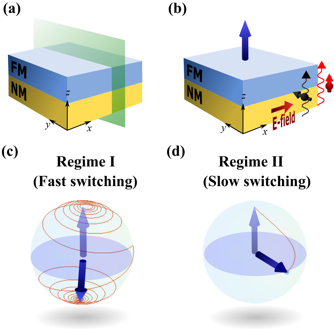
FIG. 1. (Color online) Spin Hall responses of fictitious non-magnetic (NM) slabs with varying degrees of crystalline symmetries, as exemplified by the number of mirror planes, and sample magnetization trajectories of a perpendicular ferromagnet subjected to the derived spin-orbit torques. (a) NM slab with two mirror planes M_{xz} and M_{yz} ; because the mirror plane M_{xz} is still a symmetry of the NM slab when the electric field is applied along the x direction, the spin Hall response is constrained by the remaining symmetry to produce spin currents whose flow and spin directions are mutually orthogonal to each other and the to electric field (bottom figure). (b) NM slab with single mirror plane M_{yz} ; because the electric field along the x direction breaks the only mirror plane available, the spin Hall response gives rise to conventional (black flowing spins) as well as unconventional (red flowing spins) spin currents, where the later is characterized by collinear spin and flow directions that are orthogonal to the electric field (bottom figure). (c) Bilayer heterostructure comprised of a ferromagnet (top layer) and a strong spin-orbit-coupled NM layer with a single crystalline yz mirror plane. An electric field applied along the x direction generates SOTs on the perpendicular magnetization due to conventional and unconventional spin Hall effects. The interplay between CSOT and USOT leads to the existences of distinctive dynamical regimes. The bottom figures illustrate dynamical regimes where full switching and full in-plane damping of the magnetization are expected. We note that switching to the -\hat{z} direction in regime I is faster than switching in regime II in the small intrinsic damping limit.
