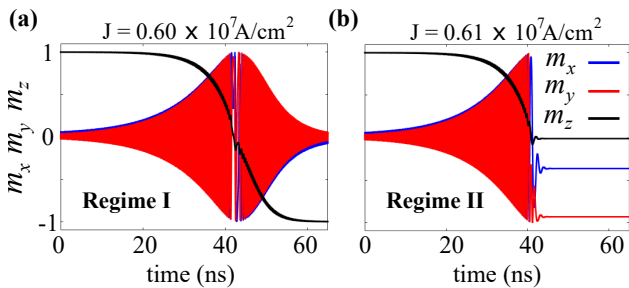
FIG. 3. (Color online) Time evolution of the components of the magnetization at a negative field-like to damping-like torque ratio of \beta = -0.2 . Upon increasing the applied current density from (a) J = 0.60 \times 10^7 A/cm 2 to (b) J = 0.61 \times 10^7 A/cm 2 , with \theta_y = 0.6 and \theta_z = 0.05 , a transition from dynamical regime I to regime II takes place.
