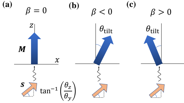
FIG. 6. (Color online) A schematic of the key factors controlling the magnetic dynamics. The magnetization (blue arrow) has an effective easy-axis which is determined by the magnetic anisotropy and the field-like torque, which tilts the magnetization from the z -axis by an amount \theta_{\text{tilt}} . The incoming spin direction (orange arrow) is determined by \theta_z/\theta_y . The squiggly arrow denotes velocity direction of spin current. The critical switching current is decreased when the magnetization and incoming spin are more aligned, as in (b).
