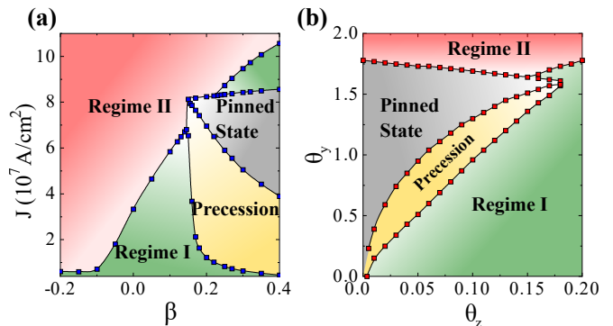
FIG. 5. (Color online) Switching diagrams of a perpendicular magnetization subjected to both CSOT and USOT. (a) current density \times field-like to damping-like torque ratio switching diagram at fixed \theta_y = 0.6 and \theta_z = 0.05 . (b) \theta_y vs \theta_z switching diagram at fixed J = 3 \times 10^7 A/cm 2 and \beta = +0.2 . Distinct dynamical regimes are represented by different colors. The boundary lines were obtained numerically by inspecting the full magnetization dynamics using the LLG equation.
