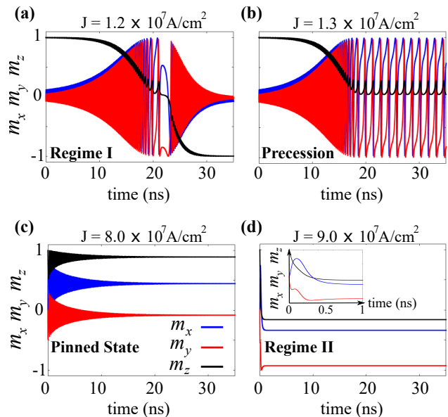
FIG. 4. (Color online) Time evolution of the components of the magnetization at a positive field-like to damping-like torque ratio of \beta = +0.2 . Here, transitions between dynamical regimes I and II take place through intermediate stable precessional and pinned state regimes: (a) J = 1.2 \times 10^7 A/cm 2 (b) J = 1.3 \times 10^7 A/cm 2 , (c) J = 8.0 \times 10^7 A/cm 2 and (d) J = 9.0 \times 10^7 A/cm 2 , with \theta_y = 0.6 and \theta_z = 0.05 .
