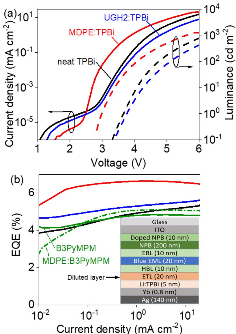
Figure 1. (a) Current density-voltage-luminance characteristics for devices with neat TPBi (black), 30 wt% MDPE:TPBi blend (red) and 30 wt% UGH2:TPBi (blue) ETLs. (b) External quantum efficiency (EQE) of the devices from panel (a), together with that from two additional devices incorporating the non-polar ETL material B3PyMPM (solid green curve) and 30 wt% MDPE:B3PyMPM (dashed green curve) for comparison. Inset: Schematic of the blue OLED architecture; only the composition of the electron transport layer (ETL) is varied between devices. Other layers in the device include the hole transport material NPB, as well as proprietary emissive, electron, and hole blocking layers (EML, EBL, and HBL, respectively).
