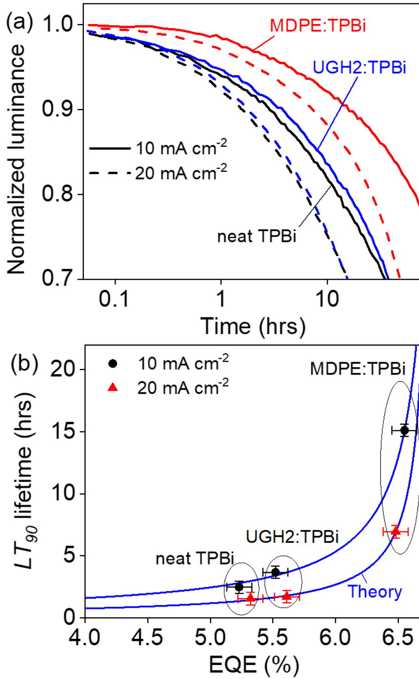
Figure 4. (a) Luminance fade results for the TPBi, UGH2:TPBi and MDPE:TPBi OLEDs at constant current densities of J = 10 and 20 \text{ mA cm}^{-2} . (b) Degradation lifetime (to 90% of initial luminance) plotted as a function of initial EQE at the fade current density, demonstrating the EPQ scaling relationship (blue lines) presented in the text.
