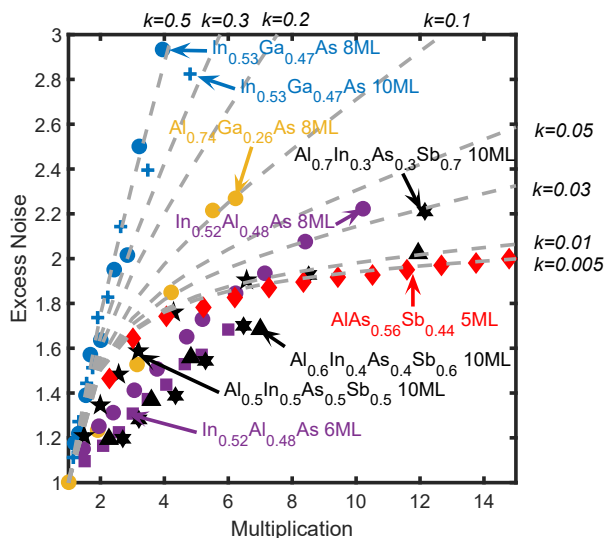
FIG. 3. Experimentally measured Excess noise vs. Multiplication gain of (In,Ga)As, (Al,Ga)As, (In,Al)As, (Al,In)(As,Sb) and Al(As,Sb) digital alloys are shown here [15–19]. The dotted lines for the corresponding k 's are plotted using McIntyre's formula [12].
