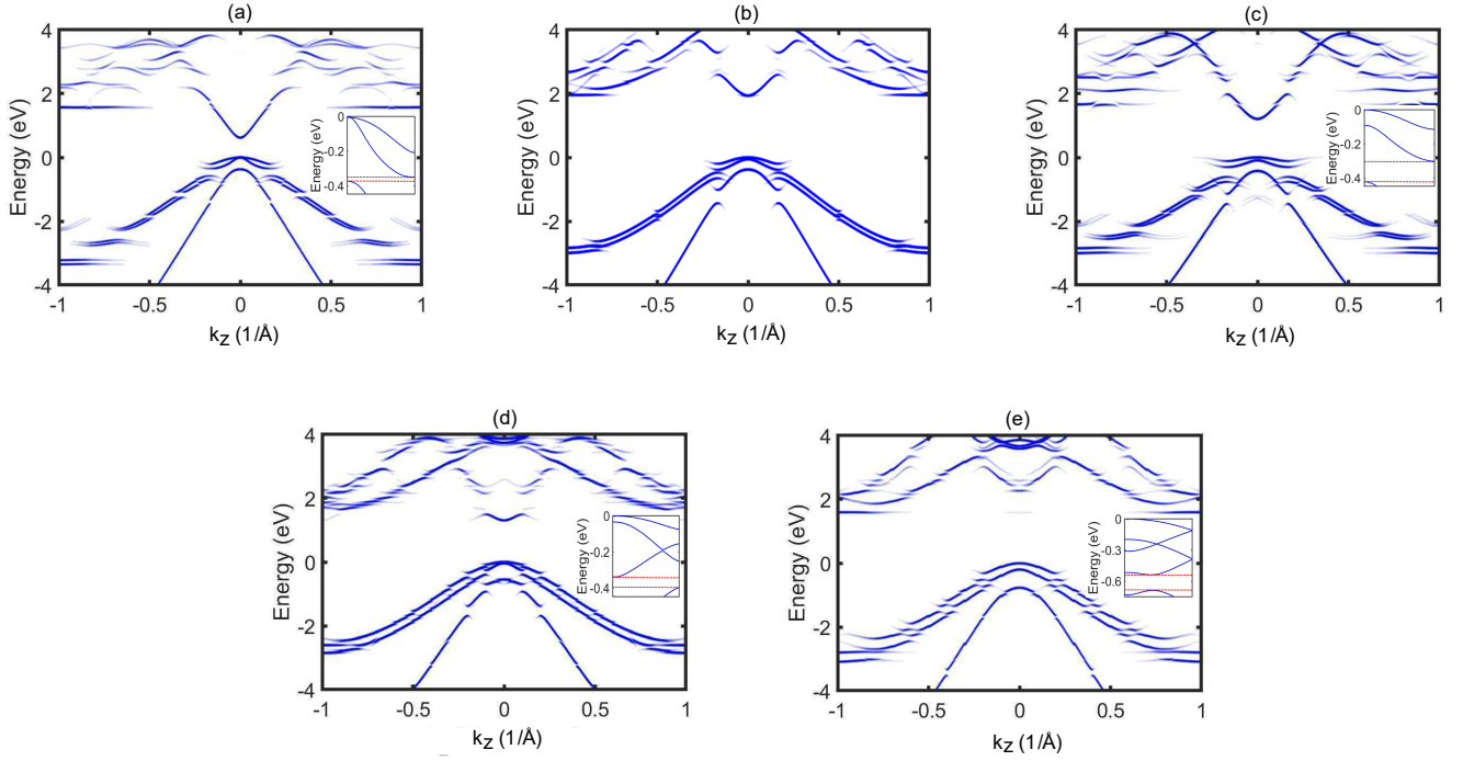
FIG. 5. Unfolded bandstructure of (a) 6ML (In,Ga)As (b) 6ML (Al,Ga)As (c) 6ML (In,Al)As (d) 10ML (Al,In)(As,Sb) (e) 5ML Al(As,Sb). The minigaps of (In,Ga)As, (In,Al)As, (Al,In)(As,Sb) and Al(As,Sb) real bandstructures are shown in the insets.
