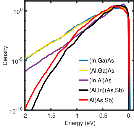
FIG. 11. Carrier density distribution vs. Energy for the valence band in the presence of optical phonon scattering computed using BTE simulation. (In,Al)As, (Al,In)(As,Sb) and Al(As,Sb) have lower occupation probability compared to (In,Ga)As and (Al,Ga)As. This prevents holes from gaining the ionization threshold energy.
