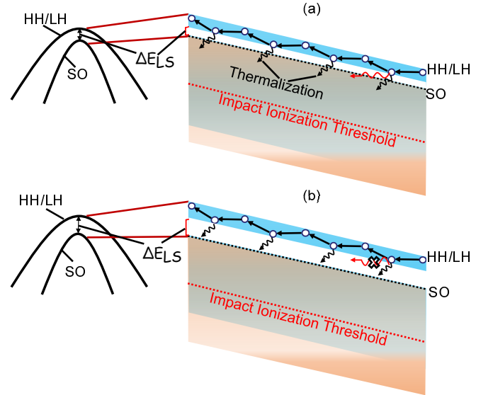
FIG. 14. Effect of spin-orbit coupling on LH/SO separation. (a) Weak coupling results in small \Delta E_{LS} and (b) strong coupling results in large \Delta E_{LS} .
