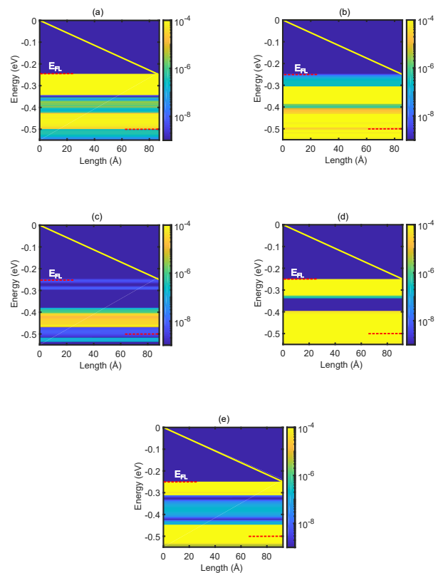
FIG. 10. Energy resolved current spectral density in the valence band for (a) (\text{In},\text{Ga})\text{As} , (b) (\text{Al},\text{Ga})\text{As} , (c) (\text{In},\text{Al})\text{As} , (d) (\text{Al},\text{In})(\text{As},\text{Sb}) and (e) \text{Al}(\text{As},\text{Sb}) . The bias for the simulation is set to V = 0.25\text{V} and total period length is 30 monolayers.
