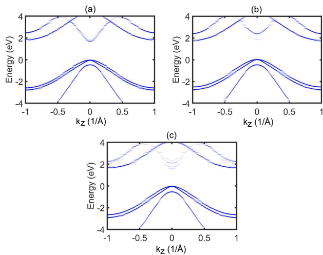
FIG. 9. Unfolded bandstructure of Sb-containing random alloys- (a) \text{Al}_{0.79}\text{In}_{0.21}\text{As}_{0.74}\text{Sb}_{0.26} , (b) \text{AlAs}_{0.44}\text{Sb}_{0.56} and (c) \text{Al}_{0.85}\text{Ga}_{0.15}\text{As}_{0.56}\text{Sb}_{0.44} .
