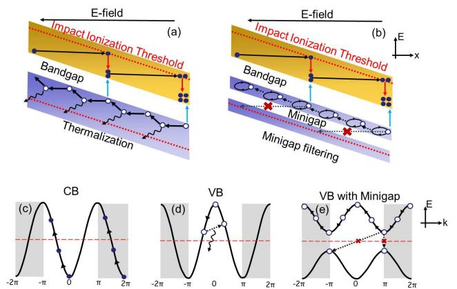
FIG. 2. Impact ionization process in normal (random alloy) APD and superlattice APD. In both APDs, it is easier for electrons to gain energy and reach the impact ionization threshold (c). The low effective mass of the electrons in these materials allow easy acceleration under applied electric field and overcome any minigaps or scattering processes present in the conduction band. In normal APDs (a), holes find it harder to gain high energy compared to electrons because of thermalization. The hole energy is reduced by thermalization due to various scattering processes as shown in (d). In superlattice APD (b), the existence of minigaps makes it harder for holes to reach higher energies. The minigaps acts as barrier that prevents holes from moving to the lower valence bands. In the plots, the y-axis E is the total energy (kinetic+potential) meaning in between inelastic scattering events the particles travel horizontally.
