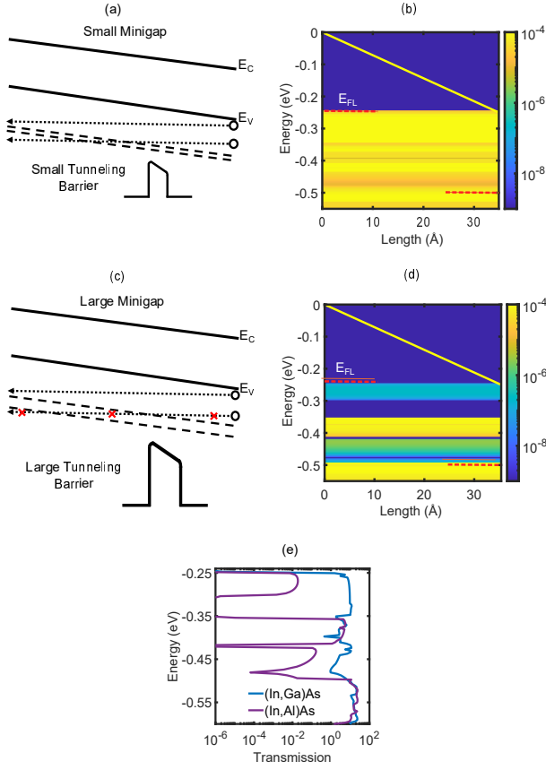
FIG. 7. Small minigaps in the valence band, as shown in (a), create a small tunneling barrier which can be overcome by holes with low mass. The spectral current density for (In,Ga)As, which has a small minigap and small LH effective mass, is shown in (b). The current spectrum for (In,Ga)As in the Fermi window is continuous. The creation of a large tunneling barrier by a larger minigap is shown in (c). This barrier prevents hole transmission. (In,Al)As has a larger minigap and LH m^* . Regions of low current density is observed within the Fermi window in the (In,Al)As spectral current density in (d). The large minigap in (In,Al)As results in reduced transmission as shown in the T(E) vs. E plot of (e). The simulations for (b), (d) and (e) were conducted under bias of V = 0.25V .
