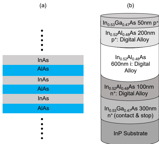
FIG. 1. (a) Digital alloy structure (b) typical structure of an APD
