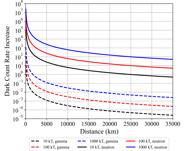
FIG. 12: DCR increase in a silicon SPAD from the prompt radiation emitted from a HANE event.
