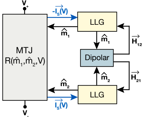
FIG. 3. Self-consistent model for the magnetization dynamics and transport: The coupled Landau-Lifshitz-Gilbert (LLG) equations provide instantaneous magnetizations to the Magnetic Tunnel Junction (MTJ) model, which in turn produces a bias-dependent spin-polarized current, \vec{I}_S(V) in the channel. +\vec{I}_S(V) is incident to one ferromagnetic interface and -\vec{I}_S(V) is incident to the other ferromagnetic interface. The dipolar model couples the two LLG solvers through fields that depend on instantaneous \hat{m}_i .
