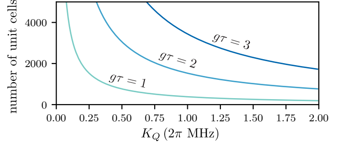
FIG. 6. Number of unit cells needed to reach g\tau in the range 1–3 as a function of self-Kerr non-linearity K_Q , for \alpha = 5 , \bar{\omega}/(2\pi) = 5 GHz, I_s = E_Q/\varphi_0 = 1.1 \mu\text{A} and Z_{\text{tml}} = 50 \Omega . The total Kerr non-linearity of the resonator K = K_Q + K_J can be tuned close to zero by introducing another non-linearity with K_J < 0 .
