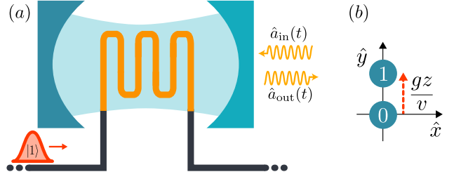
FIG. 1. (a) Sketch of the JTWPD. Standard transmission lines (black) are coupled to both ends of a one-dimensional metamaterial (orange) of length z and linear dispersion relation, \omega = vk . A cross-Kerr interaction \chi between the metamaterial and the giant probe mode (blue) leads to a phase shift in the strong measurement tone (yellow) while the signal photon (red) travels through the metamaterial. (b) Phase space picture of the probe mode. With respect to the idle coherent state |\alpha\rangle , the presence of a signal photon displaces the states by gz/v , with g = \chi\alpha .
