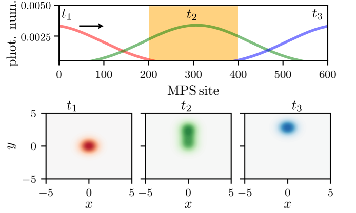
FIG. 3. The top panel shows snapshots of the photon number population along the Matrix Product State (MPS) sites at three different times t_1 (red) < t_2 (green) < t_3 (blue). The white region corresponds to the linear waveguide and the orange region to the metamaterial with its coupling to the probe resonator. The bottom three panels show the Wigner function W(x, y) of the intracavity probe field at the three respective times. When the photon is only partially inside the metamaterial, the probe is in a superposition of displaced states (middle panel). Parameters are \kappa_a = \chi(x) = K = 0 , g\tau = 2 and \gamma\tau = 2 .
