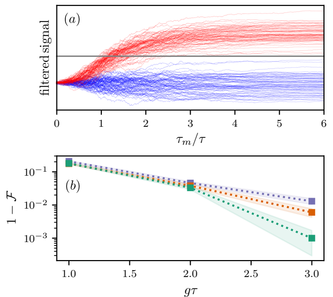
FIG. 5. (a) 75 filtered homodyne currents (arbitrary units) for g\tau = 3 , \kappa_a\tau = 1.0 , |K|/\kappa_a = 10^{-2} and g/\chi = 5 . Red traces are obtained with an incoming Gaussian photon of unitless width \gamma\tau = 6 , and blue traces for vacuum. The horizontal gray line is the threshold chosen to maximize the assignment fidelity. (b) Infidelity versus g\tau for \gamma\tau = 2 (blue), 4 (orange), and 6 (green), found by averaging over N_{\text{traj}} = 2000 trajectories. Other parameters as in (a). The shaded regions indicate the standard error defined as \pm\sqrt{\mathcal{F}(1-\mathcal{F})/N_{\text{traj}}} .
