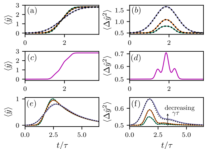
FIG. 4. Time evolution of the intra-cavity probe displacement \langle \hat{y} \rangle [(a, c, e)] and fluctuations \langle \Delta \hat{y}^2 \rangle [(b, d, f)], in the idealized case \chi(x) = K = 0 . Top row: \kappa_a = 0 and g\tau = 2 . Middle row: \kappa_a = 0 and spatially varying g(x) with average value \bar{g}\tau = 2 . Bottom row: \kappa_a\tau = 1.0 and g\tau = 2 . The solid lines correspond to MPS simulations with different photon widths \gamma\tau = 2 (blue), 4 (orange), 6 (green) and 10 (bright purple), while the dotted lines are from integrating Eq. (6).
