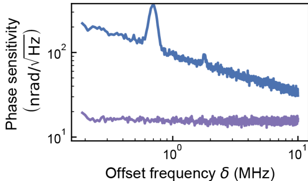
FIG. 6. Homodyne readout sensitivity. The measured readout phase resolution, due to photon shot noise is shown in purple. Additional laser phase noise leads to poorer overall resolution, shown in blue.
