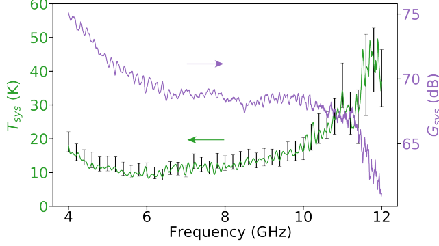
FIG. 7. System noise temperature T_{\text{sys}}(\omega) and gain G_{\text{sys}}(\omega) of the amplification chain measured using SNTJ mounted in place of JAMPA.
