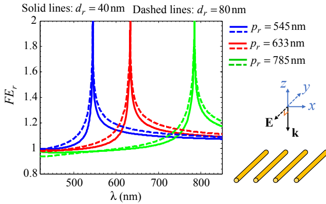
FIG. 2. Electric field enhancement FE_r achieved in the middle of the unit cell of a periodic array of gold nanorods, in a vacuum host medium, when the nanorods are excited by normal incidence plane wave polarized along the rod axis. (Field is evaluated at a point equidistant from the two adjacent rods.) Solid and dashed lines represent the result pertaining to rods' diameter of 40nm and 80 nm respectively. The period of nanorods assumed to be 545nm, 633nm and 785 nm, shown with blue, red and green respectively. Rayleigh anomaly happens at wavelength equal to the period here (normal incidence case), independent of rods diameter.
