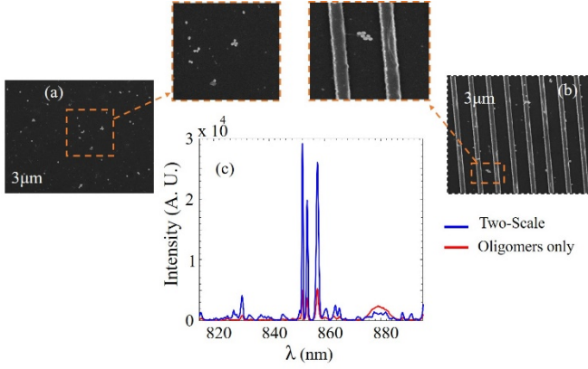
FIG 7. SEM images of gold nanosphere oligomers without nanorod array(a) and when placed within the gold nanorod array (b). In both cases, the structure is deposited on glass. The gold nanorods have a period of 900 nm and square cross section with 150nm side. The gold nanosphere oligomers are expected to have an 80 nm diameter and a 0.9 nm gap from nanosphere to nanosphere. (c) shows the SERS spectra relative to the proposed two-scale structure shown in Fig. 7(b) and to the oligomers-only structure shown in Fig. 7(a), versus wavelength. The two-scale structure provides much stronger SERS signal.
