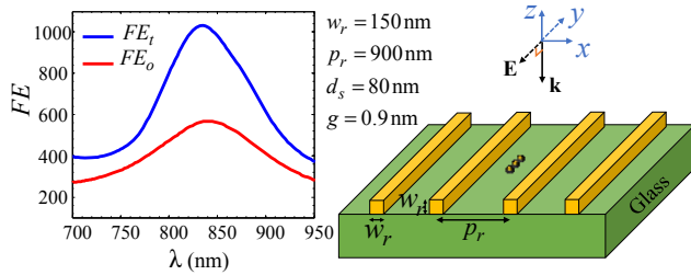
FIG. 6. Electric field enhancement versus wavelength of incident light generated by an individual gold trimer (red line) and by the combination of a periodic array of nanorods and trimer, i.e., the proposed two-scale structure (blue line). Field enhancement is calculated in the trimer hot-spot using full-wave calculations based on the FEM. The structure is located on a glass substrate, with the vacuum above. The side width of gold nanorods with square cross section is 150 nm whereas the array period is 900 nm. The diameter of gold nanospheres and the gap between them is 80nm and 0.9nm, respectively. The structure is excited by a normal-incidence plane wave polarized along the nanorods and trimer axis. For SERS application, we design our structure to attain the largest multiplicative enhancement at incident and scattered wavelength (see Eq. (13)).
