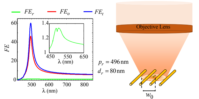
FIG. 5. Electric field enhancement versus wavelength of an incident field (a Gaussian beam), generated by: a 1-D periodic array of gold nanorods (green line), a hot-spot of an individual gold trimer (red line), and a hot-spot of a trimer located in between the array of nanorods – the two-scale structure
