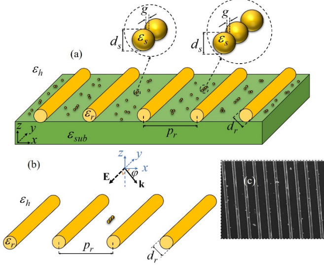
FIG. 1. (a) Proposed “two-scale” structure for enhancing the electric field at optical frequencies. It is made of oligomers of colloidal plasmonic nanospheres assembled within the nanorods of a 1-D periodic array, on top of a substrate. (b) Simplified two-scale structure for analytical investigation consisting of a representative plasmonic linear trimer in the middle of the 1-D periodic array of plasmonic nanorods in a homogeneous host medium. The orientation of the trimer is parallel to the nanorods axes and to the polarization of the incident plane wave. (c) Scanning Electron Microscopy (SEM) image of the fabricated structure, which consists of gold oligomers placed in between the periodic gold nanorods on the glass substrate. In this paper, we investigate the field enhancement in the hot-spots of the oligomers.
