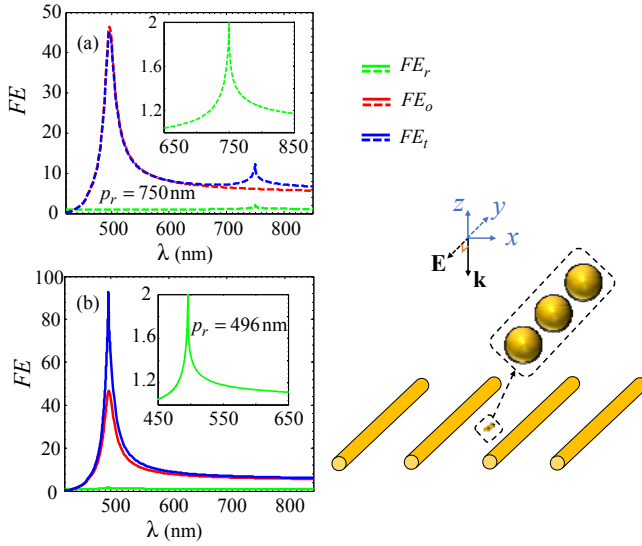
FIG. 4. Electric field enhancement versus wavelength of the incident light (polarized along the y-axis) obtained using the two-scale method, which consists of mixing a gold linear trimer placed in between the 1-D periodic array of gold nanorods. The nanorods' period and the trimer resonance plasmonic wavelength are (a) different, and (b) the same. The diameter of nanorods and nanospheres, as well as the gap between spheres, are kept constant as 80, 40 and 5 nm, respectively. The nanorod array period is p_r = 750 nm in the first case (a) and p_r = 496 nm in the second one (b). In order to achieve maximum field enhancement by the two-scale structure,
