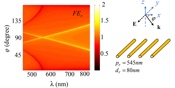
FIG. 3. Electric field enhancement FE_r versus wavelength and plane wave angle of incidence, calculated in the middle of a unit cell of the array (at the same distance from the two nearest nanorods). Gold nanorods have diameter d_r = 80 nm and period p_r = 545 nm, all supposed to be in vacuum for simplicity. The Rayleigh anomaly, responsible for the strongest enhancement, occurs at the wavelength given by Eq. (12).
