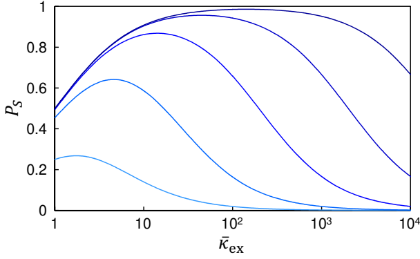
FIG. 3. Success probability P_S in Eq. (19). This holds when I_g' is negligible. Dimensionless parameter \bar{\kappa}_{\text{ex}} is defined by \bar{\kappa}_{\text{ex}} = \kappa_{\text{ex}}/\kappa_{\text{in}} . Five curves correspond to the cases where C_{\text{in}} = 1, 10, 10^2, 10^3, \text{ and } 10^4 from the bottom.
