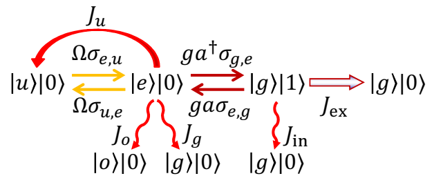
FIG. 2. Transitions in Eqs. (3) and (4).
