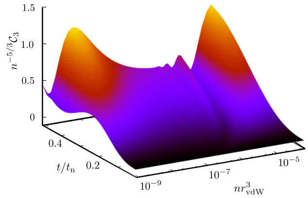
FIG. 5. Dynamical surface for the post-quench evolution of \mathcal{C}_3(t) for thermal initial conditions over a range of densities of experimental interest with \eta = 0.06 .
