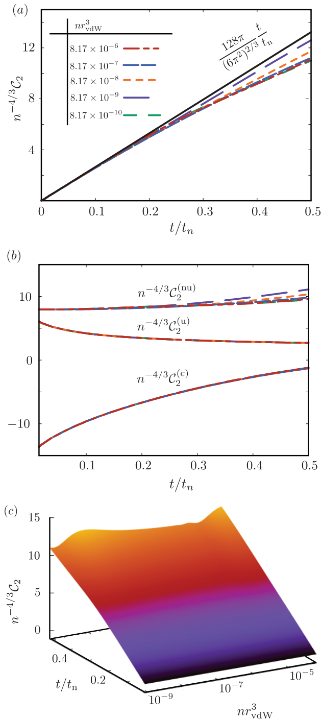
FIG. 1. (a) Dynamics of \mathcal{C}_2(t) for \eta = 0.06 for BEC initial conditions over a range of densities of experimental interest compared to the universal leading-order behavior [Eq. (27).] (b) Evolution of the components of \mathcal{C}_2(t) for the same parameters as (a). (c) Dynamical surface showing the evolution of \mathcal{C}_2(t) over a range of densities and times.
