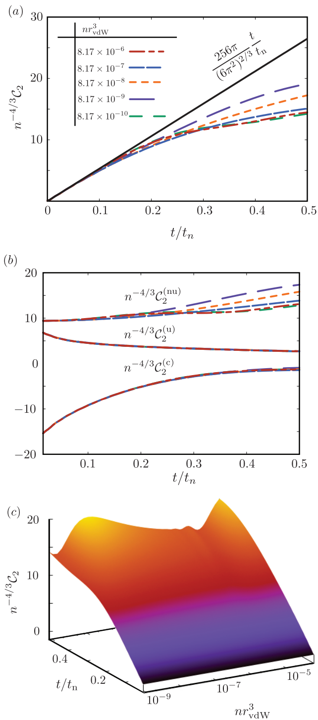
FIG. 2. (a) Dynamics of C_2(t) for thermal initial conditions with \eta = 0.06 over a range of densities of experimental interest compared to the universal leading-order behavior [Eq. (29)]. (b) Evolution of the components of C_2 over the same density range as used in (a). (c) Dynamical surface showing the evolution of C_2 over a range of densities.
