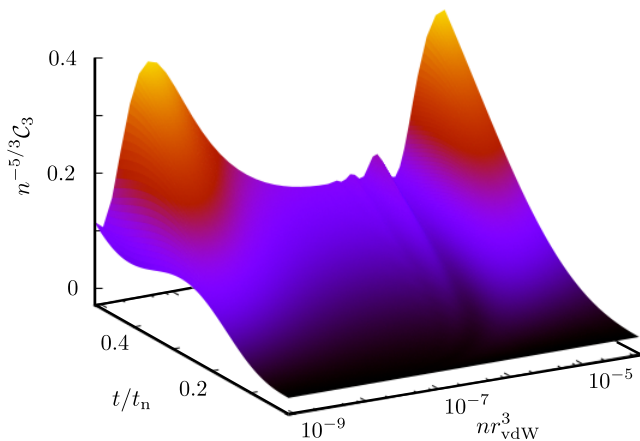
FIG. 4. Dynamical surface for the post-quench evolution of \mathcal{C}_3(t) for BEC initial conditions with \eta = 0.06 over a range of densities of experimental interest.
