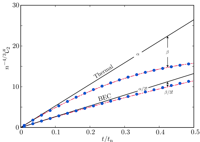
FIG. 3. Dynamics of \bar{C}_2(t) for both thermal and BEC initial conditions. The solid black lines correspond to the leading order growth formulas. The dot-dashed lines are the fits from Eqs. (32)–(33). The data points are from directly evaluating Eq. (26).
