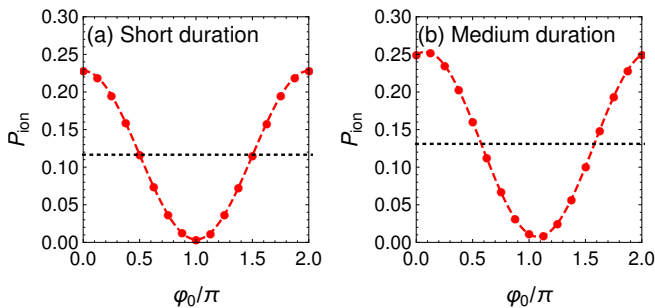
FIG. 9. Ionization probabilities for 15s + \exp(i\varphi_0)16s wave packets versus the superposition phase \varphi_0 as given in Eq. (17). Figure (a) describes a short duration pulse process with F_m = 2000 kV/cm and t_w = 606 a.u. Figure (b) describes a medium duration pulse process with F_m = 60 kV/cm and t_w = 3029 a.u., where the pulse duration is approximately one Rydberg period for 15s state: 7.0 t_w = T_{\text{Ryd}} \approx 21206 a.u. The black dotted lines are weighted averages of ionization probabilities for stationary 15s and 16s states, separately. The averages are 11.7% and 13.1% for the two processes, respectively. The red points are from quantum calculations, while the red dashed lines are their fittings. The fitting functions are 0.116 + 0.112 \cos(\varphi_0 - 0.057) and 0.130 + 0.123 \cos(\varphi_0 - 0.245) for the two processes, respectively. Details for the fitting functions can be found in the appendix.
