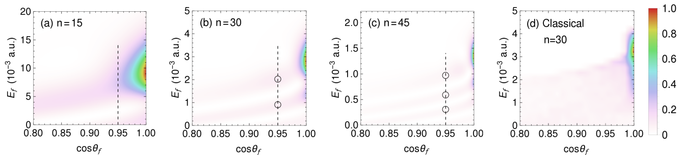
FIG. 7. The correlated energy and angular distributions with scaled pulse parameters at n = 15, 30, 45 for quantum calculations, and at n = 30 for classical calculation. The maximum densities are normalized to 1.0 for all figures. The dashed lines are at \cos\theta_f = 0.95 , while the circles are interference maxima calculated by the semiclassical method introduced in the text.
