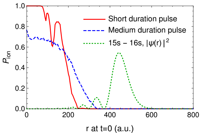
FIG. 11. Ionization probability from classical calculations versus the radial position r of electron at t = 0 . The electron is initiated at energy of n = 15 and angular momentum of zero, where the distance of the classical outer turning point is approximately 2n^2 = 450 a.u. See text for details of r . Short and medium duration pulses are defined in the caption of Fig. 9. The radial distribution from a wave packet of 15s - 16s with \varphi_0 = \pi , as shown in Fig. 8 and Eq. (17), is plotted as a reference. The radial distribution is plotted in arbitrary unit.
