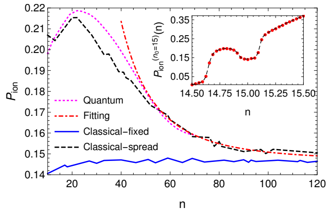
FIG. 1. Ionization probabilities from scaled classical and quantum calculations. The black dashed line is for classical calculations with an initial energy spread of n_{\text{cl}} given in Eq. (11). The blue solid line is for classical calculations at a single value of n , and the ionization probability converges to 14.6%. The magenta dotted line is for quantum calculations up to n = 70 . The red thick line is a fitting for classical results with n_{\text{cl}} spread. For n_{\text{cl}} \geq 60 , the fitting function is P_{\text{ion}} = 0.146 + 4573/n^{3.02} . The inset figure gives the classical ionization probability when the pulse parameters are fixed at n_0 = 15 and the initial classical energy state is at a single value around n_{\text{cl}} = 15 , see Eq. (14). Scaling relations are given in Eq. (13). Pulse parameters can be found in text. The initial angular momentum is fixed at l = 2 .
