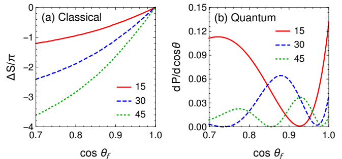
FIG. 6. Figure (a) gives the classical action differences between two paths versus the final angle, at a scaled final energy. The final energy is scaled for different n , which are E_f = (15/n)^2 \cdot 0.002 a.u. The action differences are aligned as \Delta S = 0 at \cos \theta_f = 1 . Figure (b) gives angular distributions at scaled final energies from quantum calculations.
