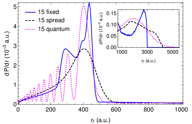
FIG. 2. Full radial distributions at the final time of the pulse, from three different calculations. The initial angular momentum is l = 2 . The blue solid curve is from a classical calculation with the initial n_{\text{cl}} fixed at 15. The black dashed curve is from a classical calculation with the initial n_{\text{cl}} being a spread of 14.5 to 15.5. The magenta dotted curve is from a full quantum calculation starting in a 15d state. The ionization probabilities from the three calculations are 14.3%, 20.7%, and 21.0%, respectively. The inset is a magnification of the distribution with r_f from 700 to 5500 a.u. Note that the probability density scale is different for the inset.
