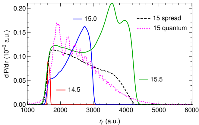
FIG. 3. Radial distributions at the final time of the pulse from classical and quantum calculations. Only those from the ionized part of the distributions are plotted. The red solid curve with small extent around 1600 a.u. is from a classical calculation with n_{cl} fixed at 14.5, and the ionization probability for this case is 0.77%. The green solid curve with the largest extent is from a classical calculation with n_{cl} fixed at 15.5, and the ionization probability for this case is 37.2%. The other three curves are the same calculations as those introduced in the caption of Fig. 2.
