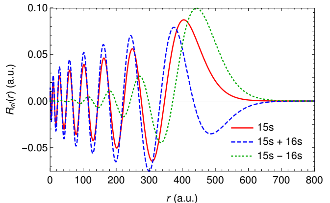
FIG. 8. Radial wave functions of the hydrogen 15s , “ 15s + 16s ”, and “ 15s - 16s ” states. Note that the 15s and 16s states do not have the equal weight ( 1/\sqrt{2} ) in the superpositions, see Eq. (17). The “ 15s + 16s ” represents a wave packet of \varphi_0 = 0 , while “ 15s - 16s ” represents \varphi_0 = \pi .
