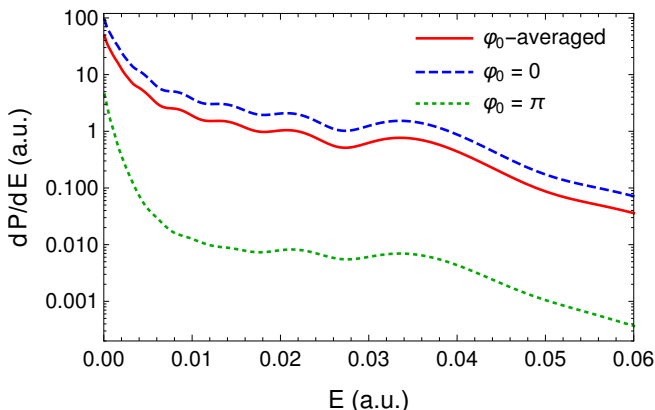
FIG. 10. Energy distributions for ionizations from 15s + \exp(i\varphi_0)16s wave packets as introduced in Eq. (17). A short duration single-cycle pulse with parameters in the caption of Fig. 9(a) is used. The results are plotted for \varphi_0 = 0, \pi , and averages of \varphi_0 ranging from 0 to 2\pi .
