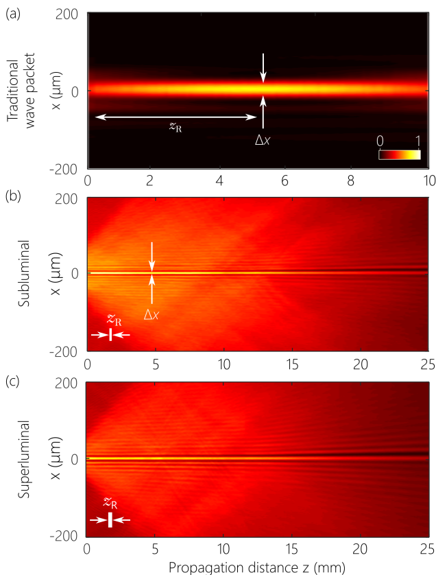
FIG. 13. Measured axial evolution of the time-averaged intensity I(x, z) for (a) a separable pulsed beam having \Delta\lambda = 8.5 nm, \Delta k_x = 0.09 rad/ \mu\text{m} , and \Delta x = 35 , \mu\text{m} , corresponding to Fig. 8(c); (b) a Class-1 ST wave packet with \theta = 30^\circ , \Delta\lambda = 2.1 nm, \Delta k_x = 0.48 rad/ \mu\text{m} , and \Delta x = 6 \mu\text{m} , corresponding to Fig. 9(a); and (c) a Class-3 ST wave packet with \theta = 60^\circ , \Delta\lambda = 2.1 nm, \Delta k_x = 0.36 rad/ \mu\text{m} , and \Delta x = 8 \mu\text{m} , corresponding to Fig. 9(c). The Rayleigh range z_R associated with the transverse width \Delta x is identified graphically in each of the three cases, and are given by (a) 4.8 mm, (b) 150 \mu\text{m} , and (c) 250 \mu\text{m} . Note the different axial (horizontal) scale used in (a) with respect to (b) and (c).
