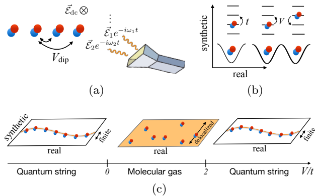
FIG. 1. (Color online) (a) Schematic illustration of the system, consisting of a 1D real-space unit-filled periodic array of polar molecules, with several microwaves illuminating them. A small dc electric (or magnetic) field may be required to detune away undesired molecular transitions. (b) The physical processes in the system. The synthetic tunneling t > 0 is driven by microwaves. The dipole interaction between molecules takes the form of a correlated tunneling process with strength V . The origin of all these processes is explained in Ref. [29]. (c) The main result of this work: The many-body ground state is a “quantum string” bound state of molecules for V/t \lesssim 0 and V/t \gtrsim 2 , and an unbound molecular gas otherwise.
