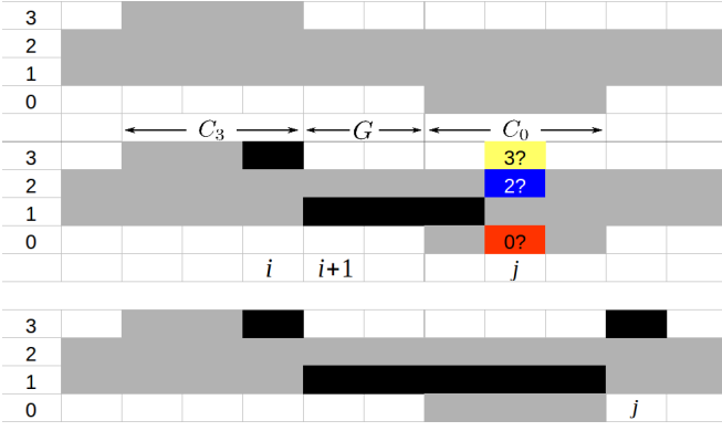
FIG. 7. Proof of Theorem 2. Top: relative positions of C_3, G, C_0 . Middle: n_j on site j is the leftmost particle on the right of site i that is not a type-1. Bottom: the case n_j = 3 , and j \notin G, j \notin C_0 .
