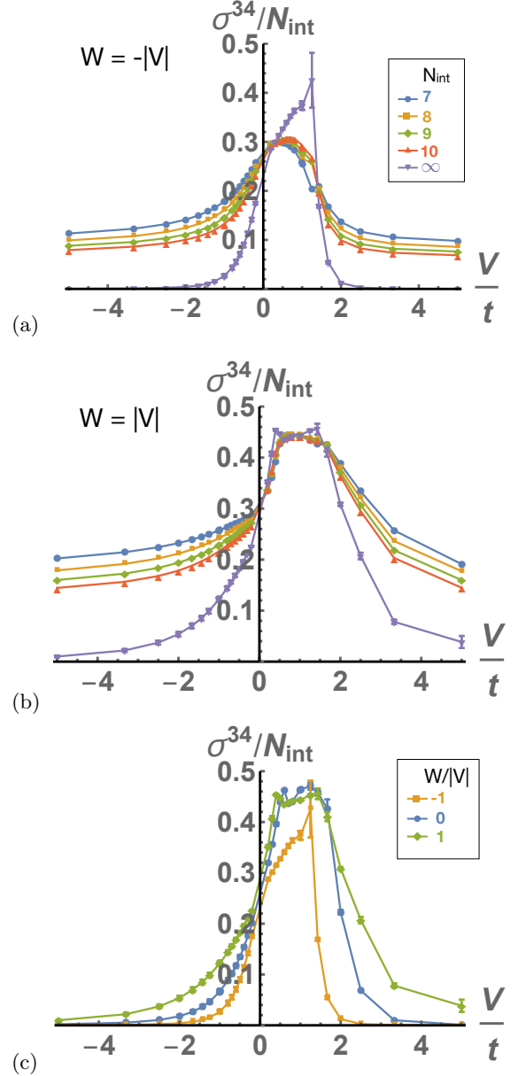
FIG. 4. (Color online) The normalized synthetic separation, \sigma^{34}/N_{\text{int}} in a 1D real-space array of N_{\text{real}} = 6 molecules and different values of N_{\text{int}} , when (a) W = -|V| , and (b) W = |V| . The extrapolated values at N_{\text{int}} \rightarrow \infty are obtained by doing a linear fit to \sigma^{34}/N_{\text{int}} vs 1/N_{\text{int}} as in Fig. 2, and the error bars indicate one standard deviation for the fit values. (c) The separation increases monotonically with W . Yellow squares: W = -|V| , blue circles: W = 0 , and green diamonds: W = |V| .
