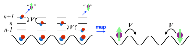
FIG. 3. (Color online) Schematic illustration of mapping the molecular system to hardcore bosons when t/V = 0 . \hat{c}_{n,j}^\dagger |\text{vac}\rangle maps to |\phi\rangle_j , and \hat{c}_{n+1,j}^\dagger |\text{vac}\rangle and \hat{c}_{n-1,j}^\dagger |\text{vac}\rangle map to \hat{b}_{\uparrow j}^\dagger |\phi\rangle_j and \hat{b}_{\downarrow j}^\dagger |\phi\rangle_j . A dipole-induced exchange of rotational states maps to tunneling of bosons. We consider only nearest-neighbor dipole interactions, although dipole interactions are longer ranged.
