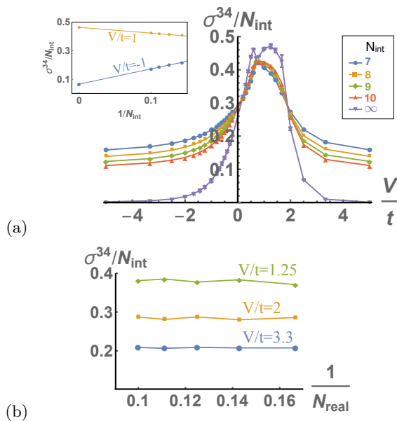
FIG. 2. (Color online) (a) The normalized synthetic separation, \sigma^{34}/N_{\text{int}} , vs V/t for different N_{\text{int}} in a 1D real-space array of N_{\text{real}} = 6 molecules. When V/t \lesssim 0 or V/t \gtrsim 2 , \sigma^{34}/N_{\text{int}} is small, and the system is therefore in the string phase. The system is in an unbound phase otherwise. The curves intersect at V/t \sim 0.2 and V/t \sim 2 , indicating that the string-gas phase transitions occur near these points. The inset shows the linear fit to the curve \sigma^{34}/N_{\text{int}} vs 1/N_{\text{int}} used to obtain the extrapolated value of \frac{\sigma^{34}}{N_{\text{int}}} at N_{\text{int}} \rightarrow \infty . The error bars indicate one standard deviation for the fit value. (b) \sigma^{34} is only weakly dependent on system size N_{\text{real}} . Blue circles, yellow squares and green diamonds show \sigma^{34}/N_{\text{int}} vs 1/N_{\text{real}} for V/t=3.3 , 2 and 1.25 and N_{\text{int}} = 6 .
