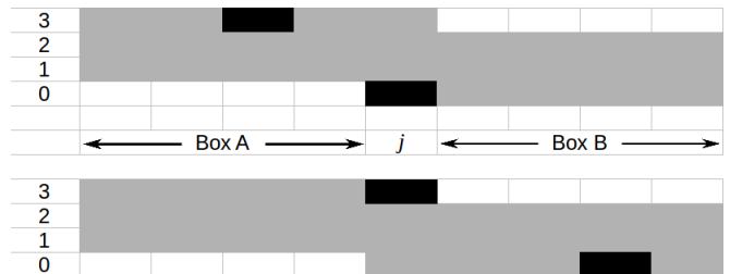
FIG. 6. Proof of Theorem 1. Here we show two different configurations in the sector S , one with a type-0 particle on real site j (top), the other with a type-3 particle on real site j (bottom). In both cases we denote the spatial region to the left of site j as "Box A", and the region to the right of site j as "Box B".
