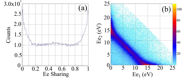
FIG. 3. Electron yield of the \text{H}^+ + \text{OH}^+ channel as a function of (a) electron energy ( E_e ) sharing ratio, E_{e1}/E_{e_{sum}} . (b) Individual electron energies.
