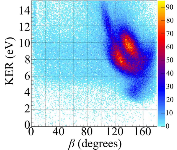
FIG. 10. H^+ + H^+ + O yield as a function of KER and \beta , dubbed nuclear conformation map.
