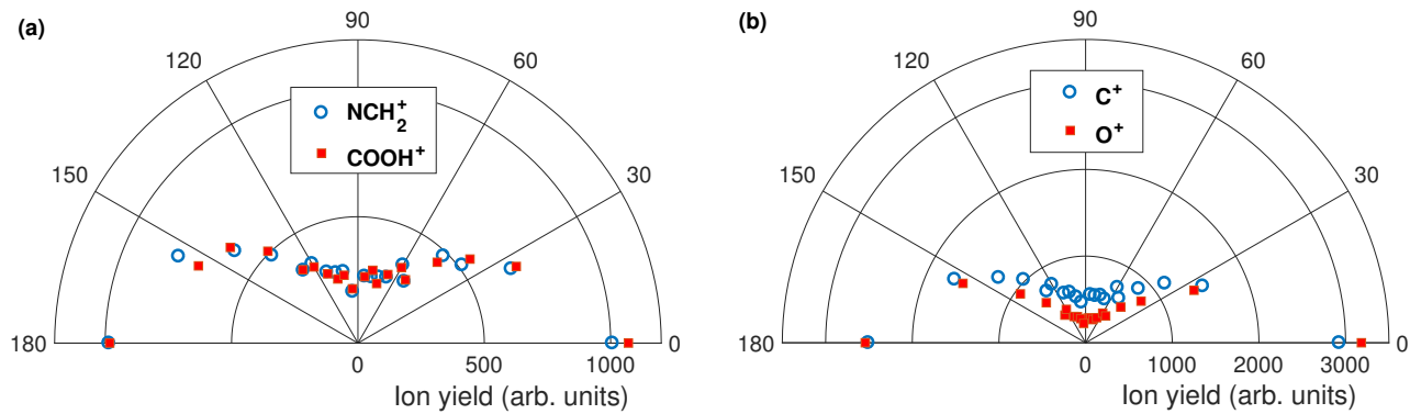
FIG. 6. (Color online) Emission angle distribution of ion-ion coincidence between m=28 and m=45 and coincidence between m=12 and m=16 . The distributions are normalized to peak values at 180^\circ . The legends show the ion species of the dominant contribution to fragment ion yields.
