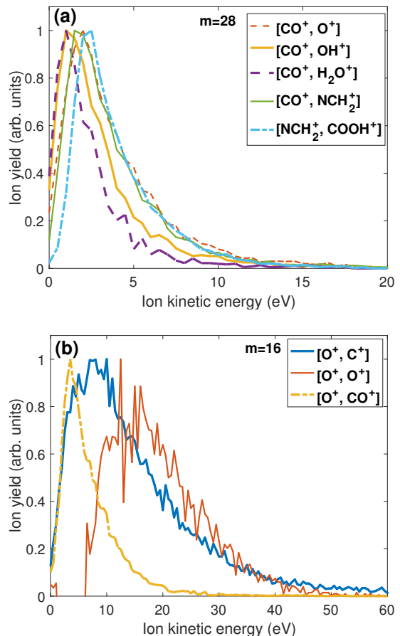
FIG. 4. (Color online) Kinetic energy (KE) distributions of (a) m=28 and (b) m=16 from different ion-ion coincidence channels. Spectra are normalized to the peak height. In (b) the contribution from the residual background gas was subtracted for self-coincidence of m=16 ; for all other coincidence channels, the contribution by the residual background gas was insignificant and can be neglected. The legends show the ion species of the dominant contribution to fragment ion yields.
