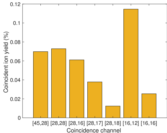
FIG. 3. (Color online) Coincident ion pair yields normalized to the total coincident ion yield. Coincident events resulting from the ionization of the residual gas were subtracted.
