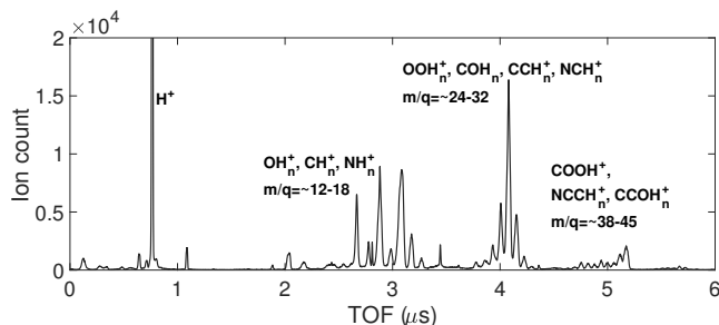
FIG. 1. (Color online) Time of flight (TOF) spectrum of glycine irradiated with x-ray at 310 eV.
