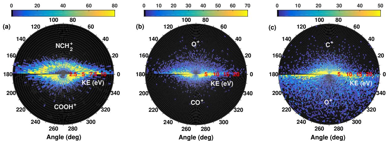
FIG. 8. (Color online) Correlation between KE and the ion emission angle, relative to the x-ray polarization. The upper and lower half-circles show the maps for the lighter and heavier fragments, correspondingly. The color represents the abundance of the ions (see color bars). (a) Coincidence between m=28 and m=45 ; (b) coincidence between m=16 and m=28 ; (c) coincidence between m=12 and m=16 .
