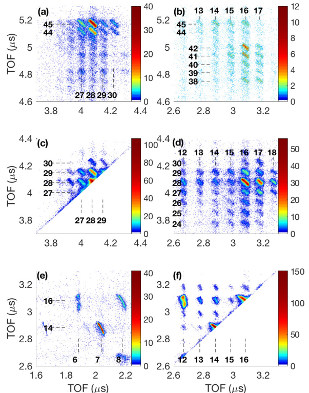
FIG. 2. (Color online) Photoion-Photoion coincidence (PIPICO) false-color map of glycine. Panels (a)-(f) show different regions of the time-of-flight range covered by the experiment. Dashed lines and labels indicate the corresponding m/q positions. The coincidence counts color scale is given at the right of all the panels. See details in the text.
