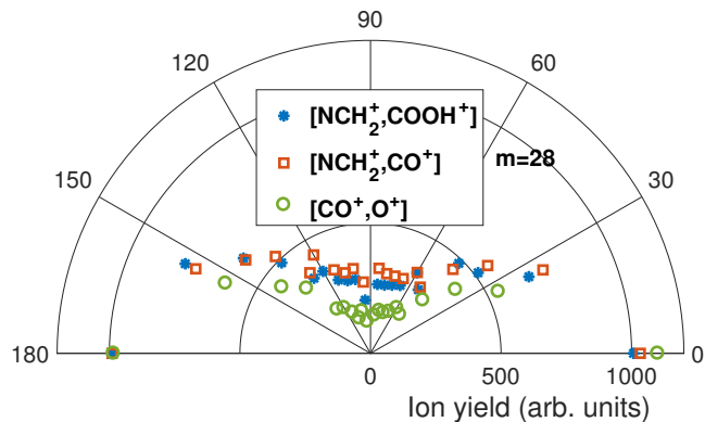
FIG. 5. (Color online) Emission angle distribution of ion with m=28 associated with different dissociation channels. The angle is relative to the polarization direction of the x-rays. The distributions are normalized to peak values at 180^\circ . The legends show the ion species of the dominant contribution to fragment ion yields.
