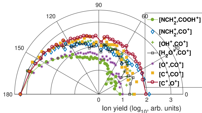
FIG. 7. (Color online) Dissociation angle distribution of coincident fragment ions for different fragmentation channels, normalized to the highest values. The distributions are normalized to peak values at 180^\circ . The ion yields are presented in log scale (see radial axis label) for clarity. The legend shows the main fragmentation channel to which the given fragments are assigned.
