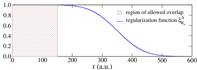
FIG. 1: Function \xi_{R_0}^\Delta(r) with R_0 = 350 a.u. and \Delta = 100 a.u. employed in this study to regularize the free-free dipole moments expressed in the length form. The dashed domain represents the region where bound and free functions can overlap.
