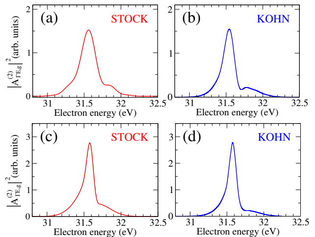
FIG. 6: Two-photon ionization probability from helium ground state to the final \Gamma = ^1S state at SB_{-1} calculated using both STOCK and Kohn methods. The optical pulse has intensity 2.5 \times 10^{11} W/cm 2 , wavelength 300 nm, and FWHM 30 fs in (a) and (b), and 50 fs in (c) and (d).
