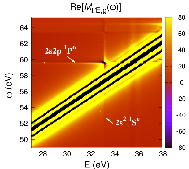
FIG. 4: Real part of \mathcal{M}_{\Gamma E, g}(\omega) for a two-photon transition to the final ^1S electronic state leading to ^2\text{He}^+(1s) product as a function of the final electron energy E and the photon frequency \omega .
