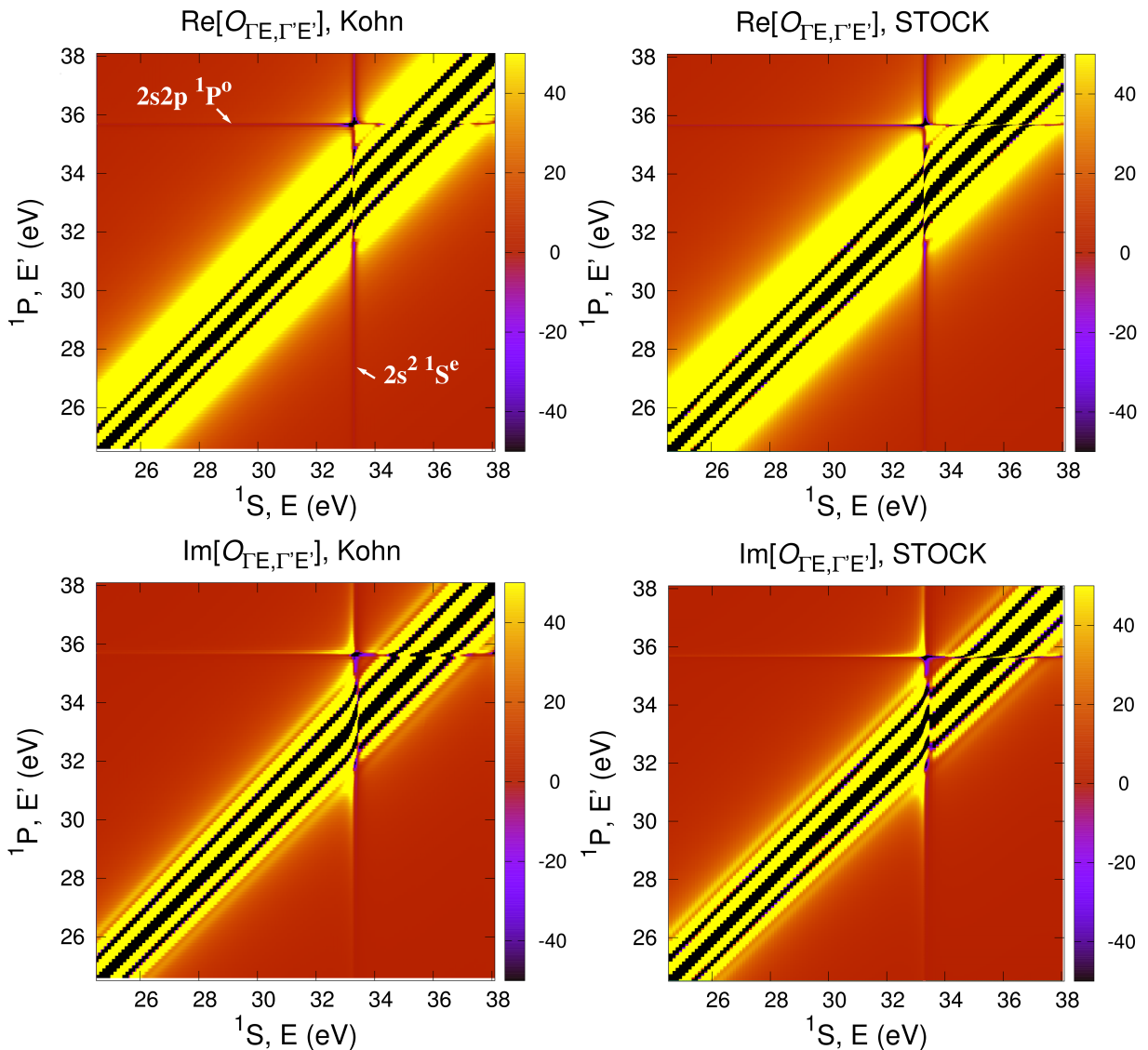
FIG. 3: Real (upper panels) and imaginary (lower panels) parts of the free-free transition dipole moments \mathcal{O}_{\Gamma E, \Gamma' E'} as a function of E' and E , from the ^1P to ^1S symmetries, calculated in the length gauge, using the Kohn (left panels) and the velocity gauge STOCK (right panels) methods (see text for details).
