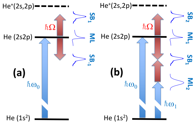
FIG. 5: Ionization schemes considered in this study: (a) two-photon ionization with a combined XUV and IR/optical field, and (b) RABBITT-like scheme with two XUV pulses with frequencies, \omega_0 and \omega separated by twice the IR frequency.
