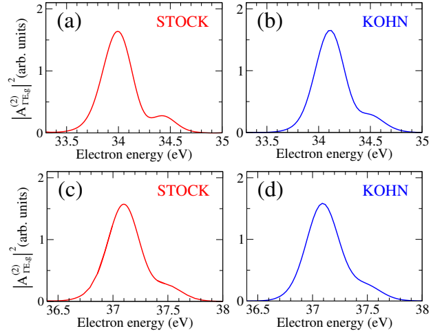
FIG. 8: Same as Fig. 7 for an infrared pulse with wavelength 800 nm and FWHM 13 fs.
