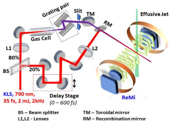
FIG. 2. (Color online) Sketch of the experimental setup.
