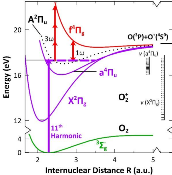
FIG. 1. (Color online) A sketch of potential energy curves (PECs) for the ground state of O 2 (taken from Ref. [37]) and selected low-lying states of O 2 + (adapted from Ref. [38]). The purple arrow depicts the EUV-induced photoionization at the equilibrium distance of the neutral molecule, whereas the red arrows indicate the positions of 3\omega and 1\omega resonant transitions between a^4\Pi_u to the f^4\Pi_g states [39]. Dashed tick marks on the right indicate the energies of accessible vibrational levels for the X^2\Pi_g and a^4\Pi_u ionic states. The most abundant vibrational levels in the Franck-Condon region are highlighted with thicker black lines for both states.
