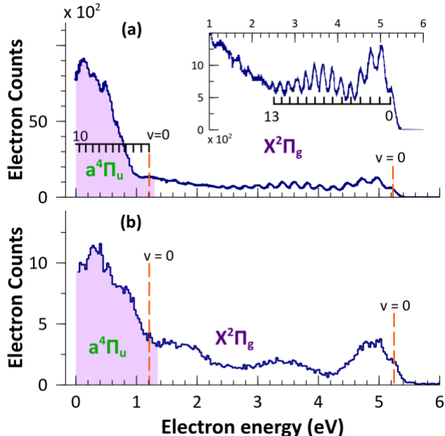
FIG. 3. (Color online) The measured photoelectron energy distribution for photoionization of O_2 by the 11 th harmonic EUV with a bandwidth of \leq 200 meV (a) and \sim 300 meV (b). The inset in (a) shows the enlarged view of the region corresponding to the X^2\Pi_g ground state.
