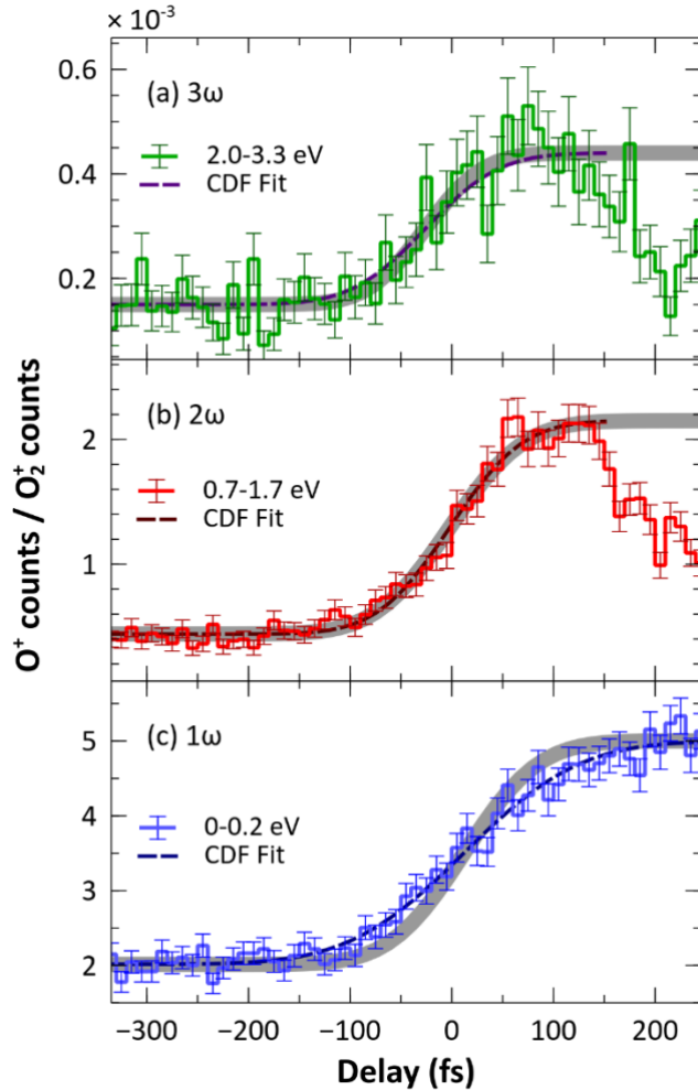
FIG. 7. (Color online) Delay-dependent ratio of O^+ to O_2^+ yields for three different KER regions associated with 3\omega , 2\omega and 1\omega transitions, respectively: (a) 2-3.3 eV; (b) 0.7-1.7 eV; (c) 0-0.2 eV. Dashed lines represent the Gaussian CDF fits to the data. Shaded gray line in all panels depicts the CDF with the Gaussian width of \sigma = 57 fs corresponding to the measured cross-correlation of the EUV and NIR pulses (identical to the CDF shown in Fig. 4(b)).
