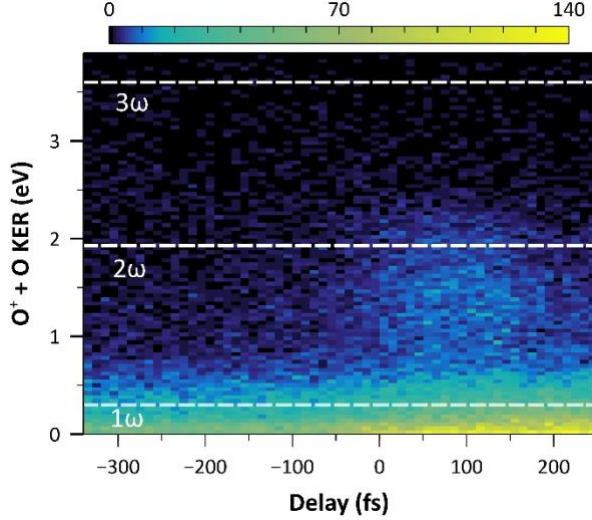
FIG. 6. (Color online) The measured KER distribution for O+O + dissociation fragments as a function of EUV-IR delay. The dashed lines separate the contributions from different channels corresponding to the KER regions indicated in Fig. 5.
