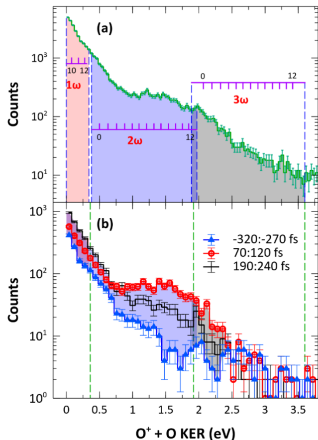
FIG. 5. (Color online) (a) Kinetic energy release (KER) distribution of the O+O^+ channel integrated over all EUV-IR delays. Vertical dashed lines indicate the KER values expected for O_2^+ dissociation via 1\omega , 2\omega and 3\omega transitions from different vibrational levels of the a^4\Pi_u to the f^4\Pi_g state at 790 nm. Shaded areas depict the range of KER expected for each transition considering the bandwidth of the NIR probe pulse. (b) KER distributions for three different EUV-NIR delay regions.
