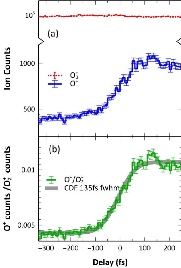
FIG. 4. (Color online) (a) The measured yields of O_2^+ (dotted red line) and O^+ (solid blue line) ions as a function of EUV-NIR delay. (b) The measured ratio of O^+ / O_2^+ yields as a function of EUV-NIR delay. The shaded grey line depicts the Gaussian cumulative distribution function (CDF) corresponding to the overlap between the EUV and NIR pulses defined from their measured cross-correlation (see text).
