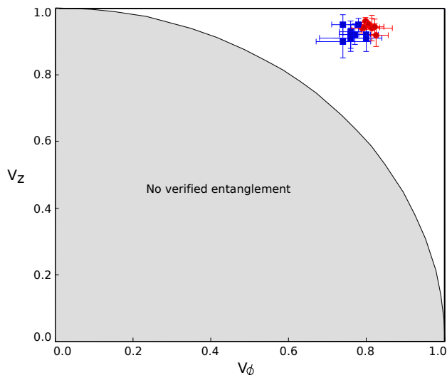
FIG. 6. (Color online) Entanglement verification. The Negative Partial Transpose (NPT) criterion [32, 33] is used to obtain the required entanglement visibilities, certifying the presence of entanglement in an arbitrary 2 \times 3 -dimensional quantum state. Our experimental results for various angles with Method 1 (red circles) and Method 2 (blue squares) are well above the classical bound (black line).
